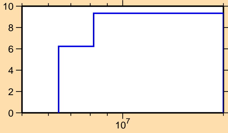
\Delta\sigma/\sigma vs. E for ^{38}\text{S}(n,n_1)
