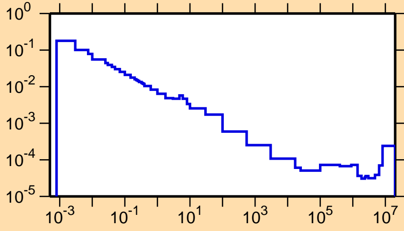
\sigma vs. E for ^{38}\text{S}(n,\gamma)
