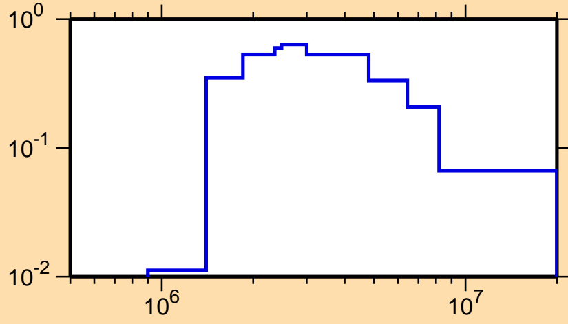
\sigma vs. E for ^{38}\text{S}(n,n_1)
