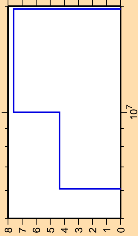
\Delta\sigma/\sigma vs. E for ^{40}\text{S}(n,2n)
