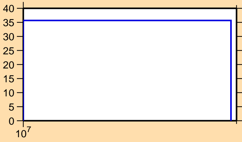
\Delta\sigma/\sigma vs. E for ^{40}\text{S}(n,ncont.)
