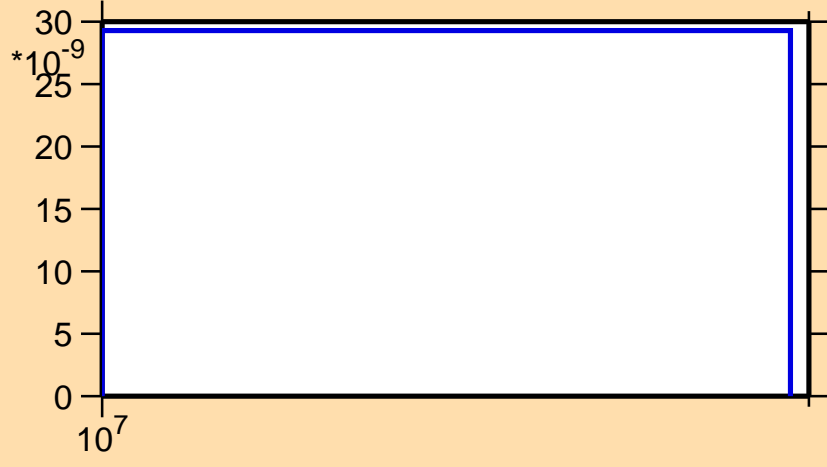
\sigma vs. E for ^{40}\text{S}(n,t)
