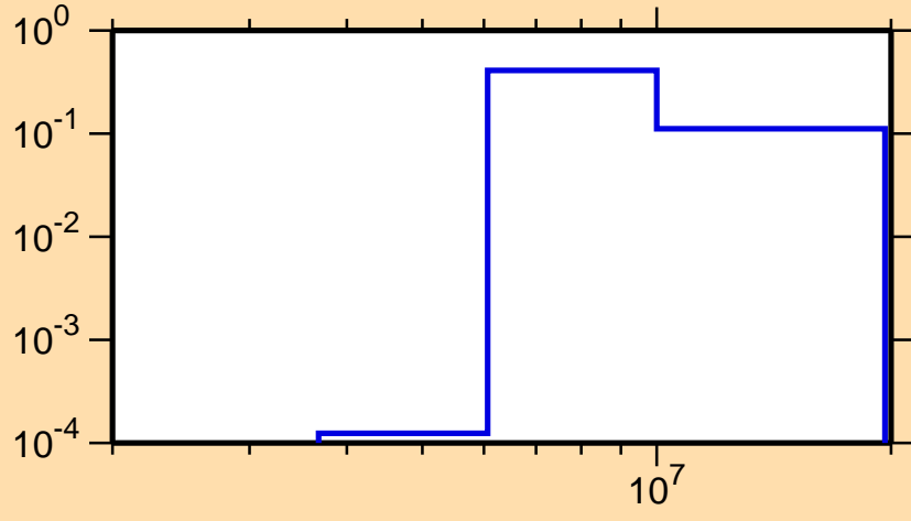
\sigma vs. E for ^{40}\text{S}(n,n\text{cont.})
