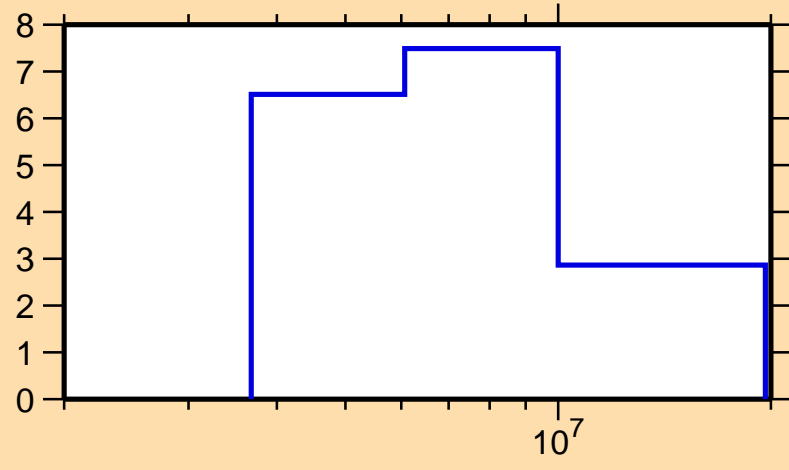
\Delta\sigma/\sigma vs. E for ^{40}\text{S}(n,el.)
