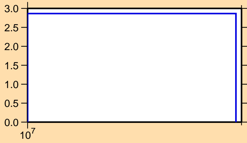
\Delta\sigma/\sigma vs. E for ^{40}\text{S}(n,el.)
