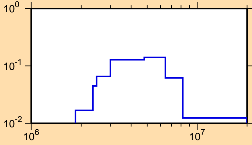
\sigma vs. E for ^{40}\text{S}(n,n_2)
