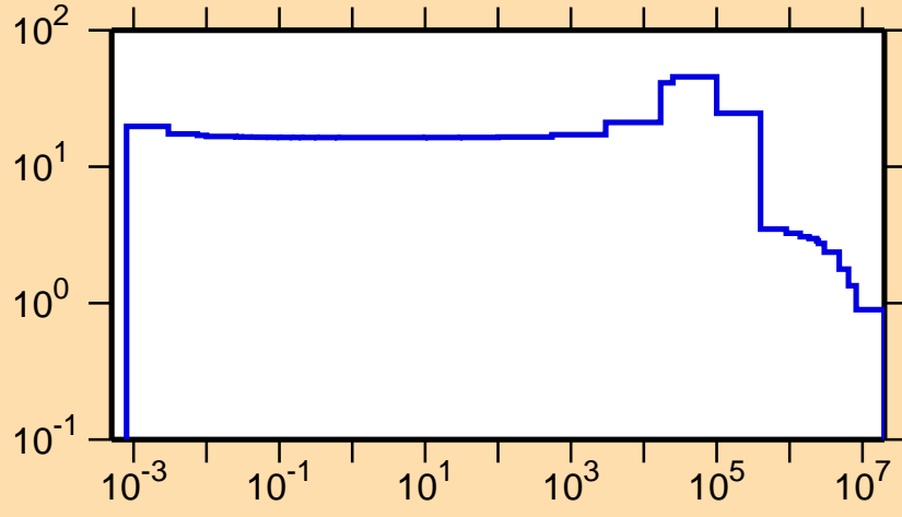
\sigma vs. E for ^{40}\text{S}(n,\text{el.})
