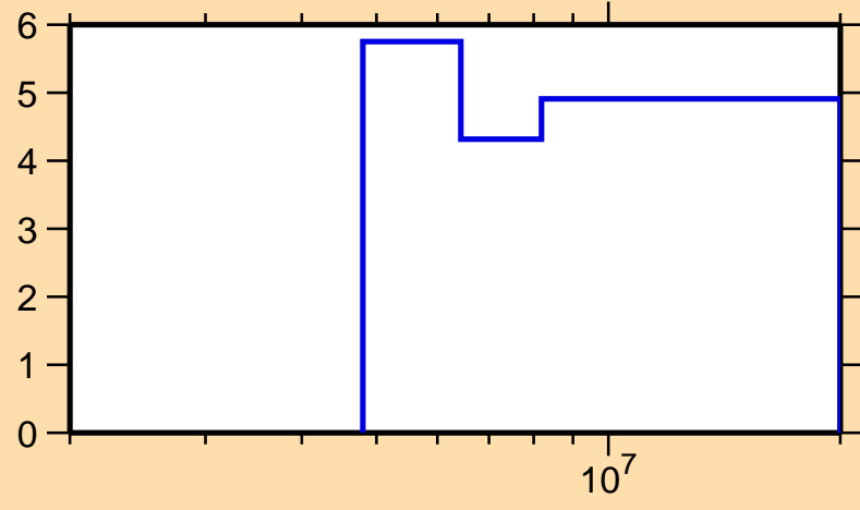
\Delta\sigma/\sigma vs. E for ^{40}\text{S}(n,n\text{onel.})
