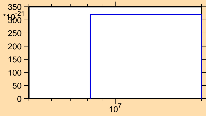
\sigma vs. E for ^{40}\text{S}(n,2n\alpha)
