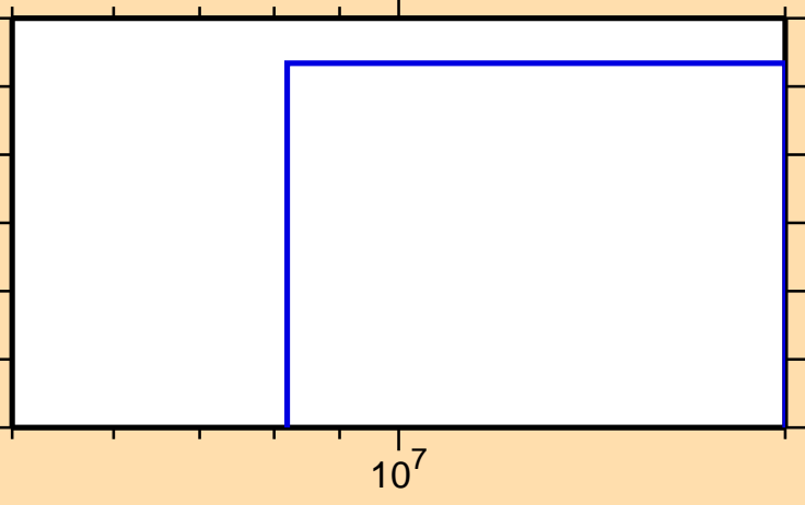
\sigma vs. E for ^{40}\text{S}(n,n\alpha)
