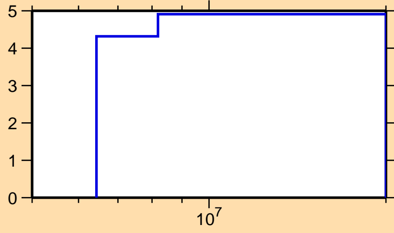
\Delta\sigma/\sigma vs. E for ^{40}\text{S}(n,\text{nonel.})
