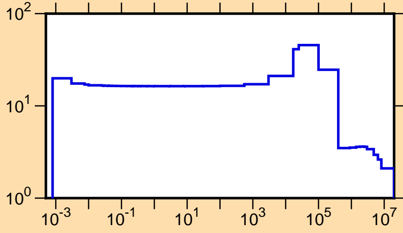
\sigma vs. E for ^{40}\text{S}(n,\text{tot.})
