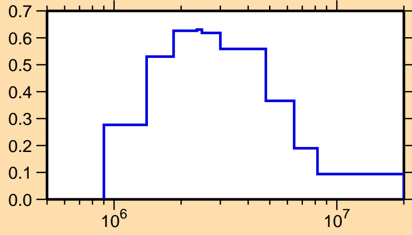
\sigma vs. E for ^{40}\text{S}(n,n_1)
