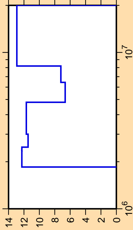
\Delta\sigma/\sigma vs. E for ^{40}\text{S}(n,n_2)
