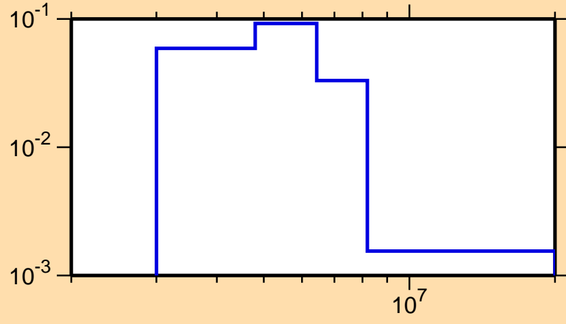
\sigma vs. E for ^{40}\text{S}(n,n_4)
