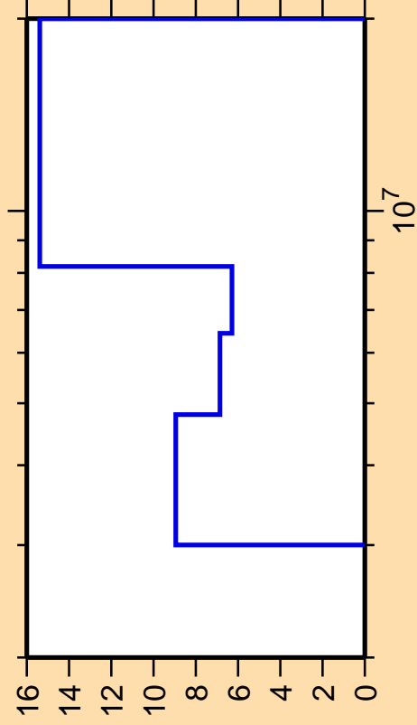
\Delta\sigma/\sigma vs. E for ^{40}\text{S}(n,n_4)
