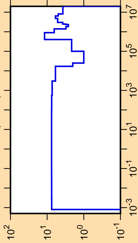
\Delta\sigma/\sigma vs. E for ^{40}\text{S}(n,\text{tot.})
