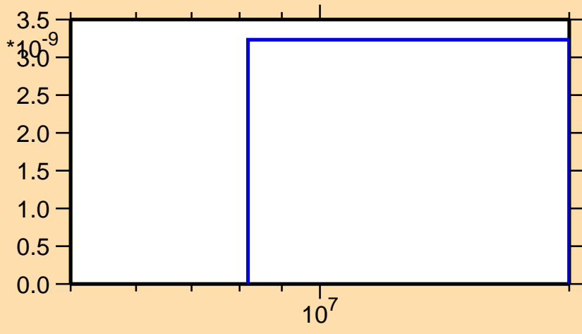
\sigma vs. E for ^{40}\text{S}(n,np)
