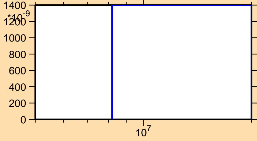
\sigma vs. E for ^{40}\text{S}(n,\alpha)
