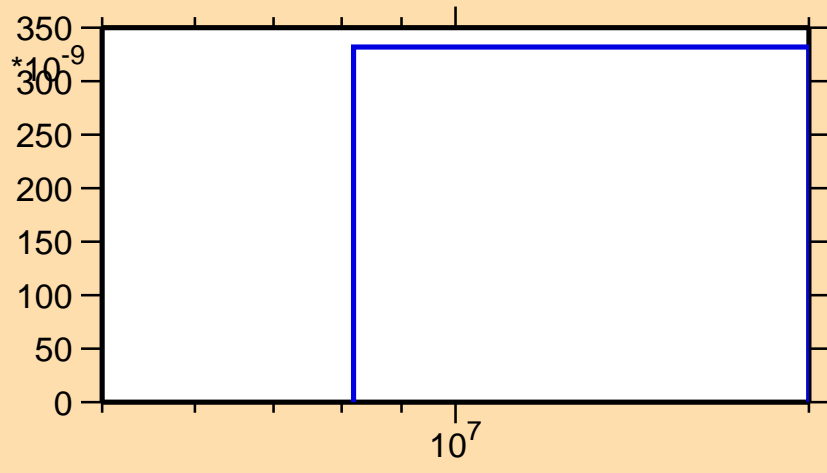
\sigma vs. E for ^{40}\text{S}(n,p)
