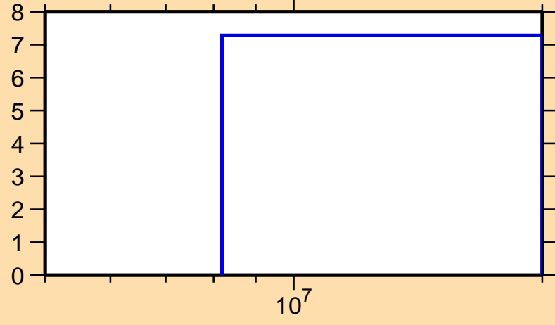
\Delta\sigma/\sigma vs. E for ^{40}\text{S}(n,2n)
