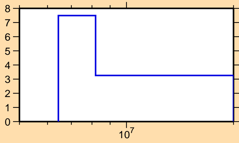
\Delta\sigma/\sigma vs. E for ^{40}\text{S}(n,\text{el.})
