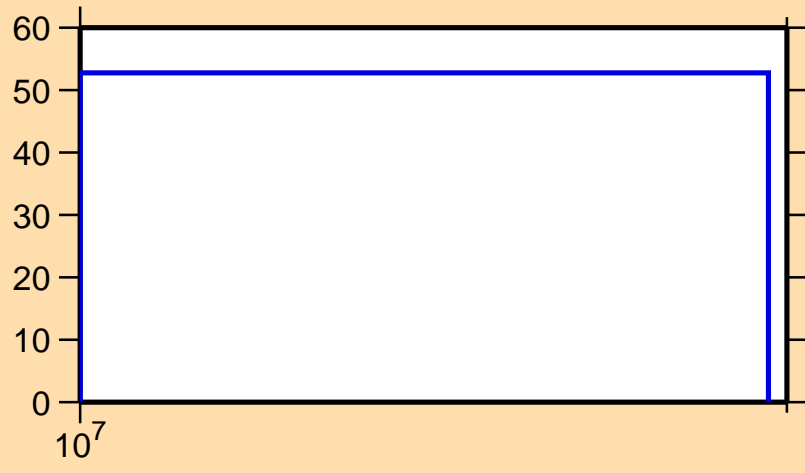
\Delta\sigma/\sigma vs. E for ^{41}\text{S}(n,p)
