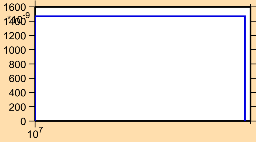
\sigma vs. E for ^{41}\text{S}(n,t)
