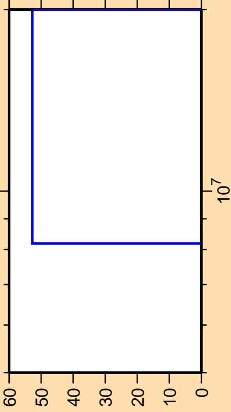
\Delta\sigma/\sigma vs. E for ^{41}\text{S}(n,p)
