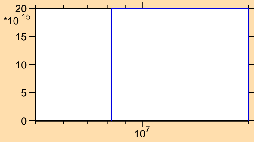
\sigma vs. E for ^{41}\text{S}(n,nt)
