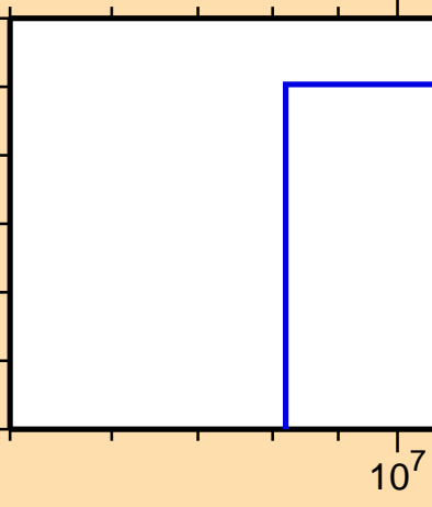
\sigma vs. E for ^{41}\text{S}(n,n\alpha)
