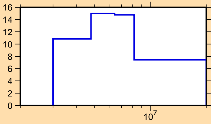
\Delta\sigma/\sigma vs. E for ^{41}\text{S}(n,el.)
