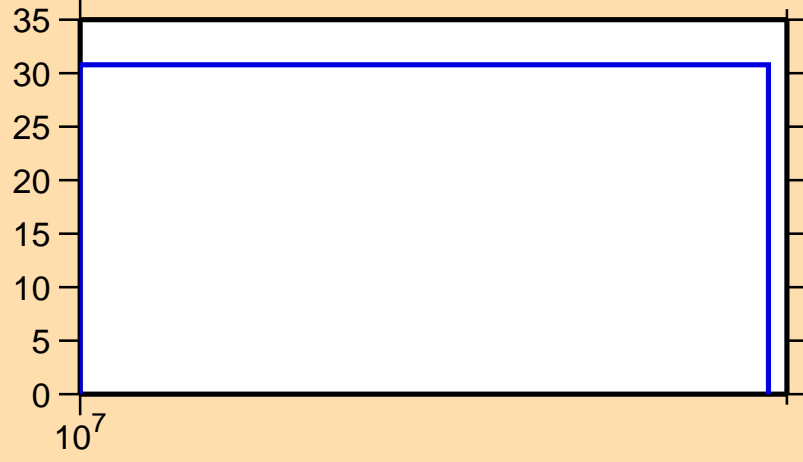
\Delta\sigma/\sigma vs. E for ^{42}\text{S}(n,inel.)
