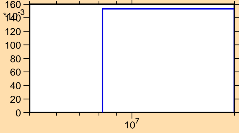
\sigma vs. E for ^{42}\text{S}(n,3n)
