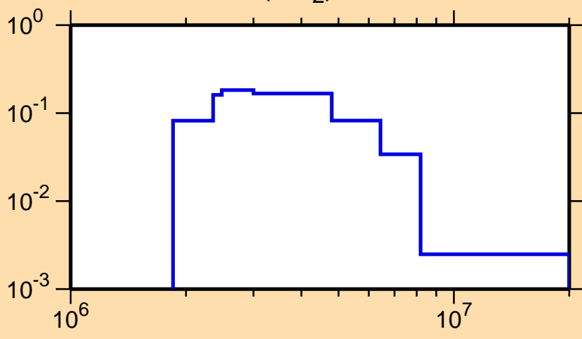
\sigma vs. E for ^{42}\text{S}(n,n_2)
