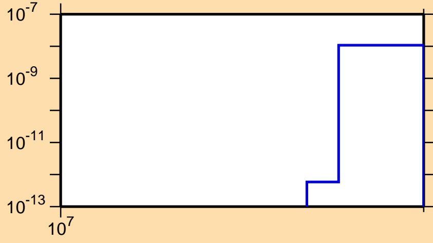
\sigma vs. E for ^{107}\text{Sb}(n,nt)
