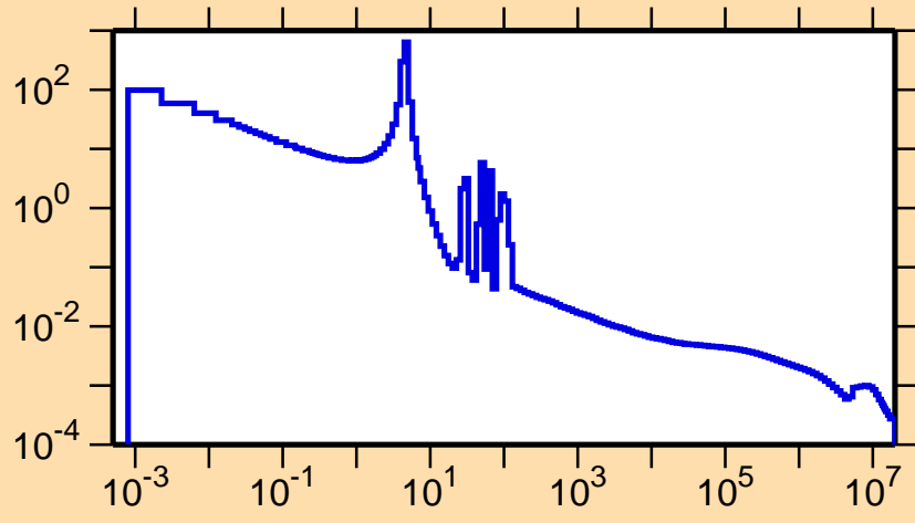
\sigma vs. E for ^{107}\text{Sb}(n,\gamma)
