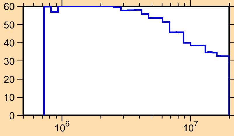
\Delta\sigma/\sigma vs. E for ^{107}\text{Sb}(n,n_1)
