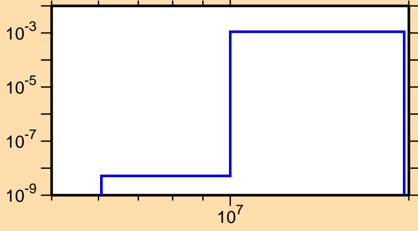
\sigma vs. E for ^{107}\text{Sb}(n,\text{pd})
