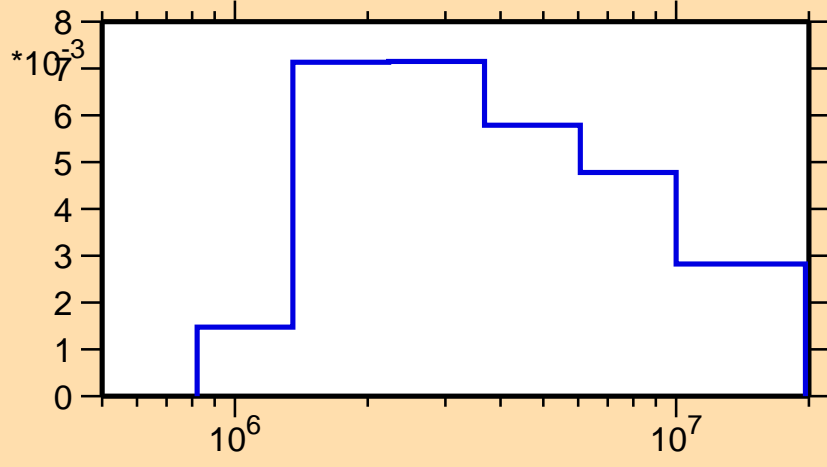
\sigma vs. E for ^{107}\text{Sb}(n,n_2)
