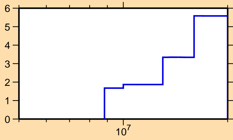
\Delta\sigma/\sigma vs. E for ^{108}\text{Sb}(n,\text{tot.})
