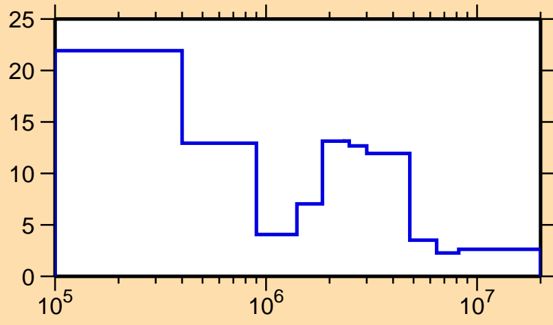
\Delta\sigma/\sigma vs. E for ^{108}\text{Sb}(n,\text{tot.})
