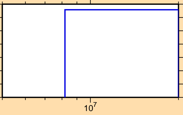
\sigma vs. E for ^{108}\text{Sb}(n,\text{pt})
