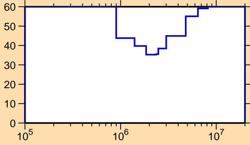
\Delta\sigma/\sigma vs. E for ^{108}\text{Sb}(n,n_1)
