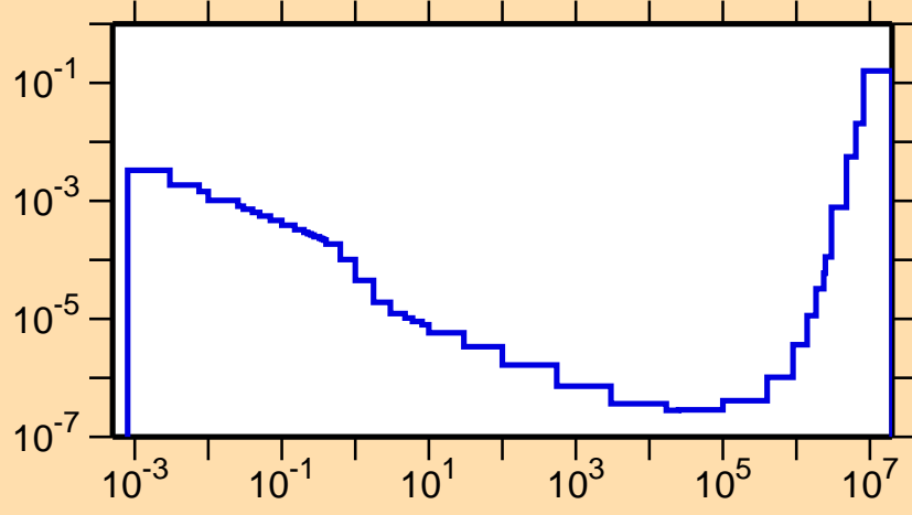
\sigma vs. E for ^{108}\text{Sb}(n,p\alpha)
