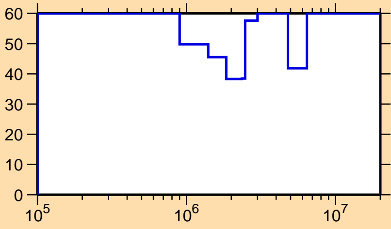
\Delta\sigma/\sigma vs. E for ^{108}\text{Sb}(n,\text{inel.})
