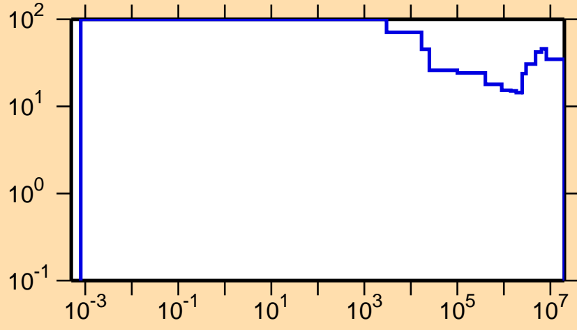
\Delta\sigma/\sigma vs. E for ^{108}\text{Sb}(n,p)
