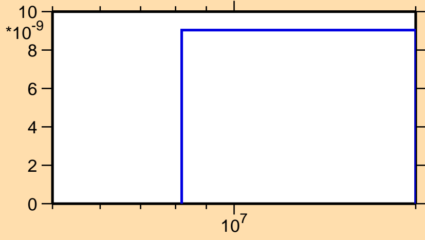
\sigma vs. E for ^{108}\text{Sb}(\text{mt } 34)
