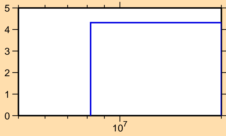
\Delta\sigma/\sigma vs. E for ^{108}\text{Sb}(n,\text{el.})
