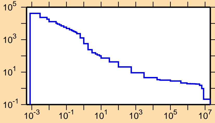
\sigma vs. E for ^{108}\text{Sb}(n,p)
