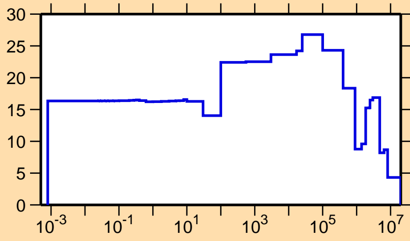
\Delta\sigma/\sigma vs. E for ^{108}\text{Sb}(n,\text{el.})
