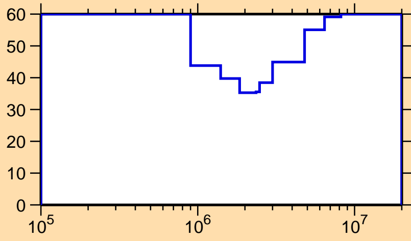
\Delta\sigma/\sigma vs. E for ^{108}\text{Sb}(n,n_1)
