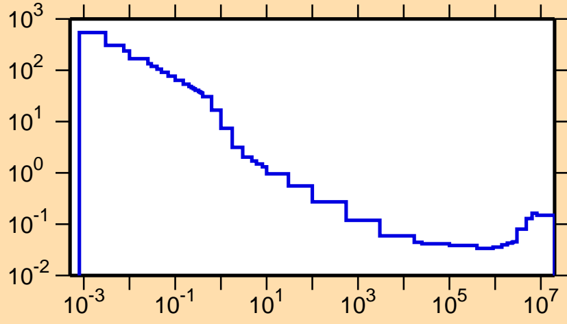
\sigma vs. E for ^{108}\text{Sb}(n,\alpha)
