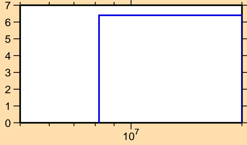
\Delta\sigma/\sigma vs. E for ^{108}\text{Sb}(n,\text{nonel.})
