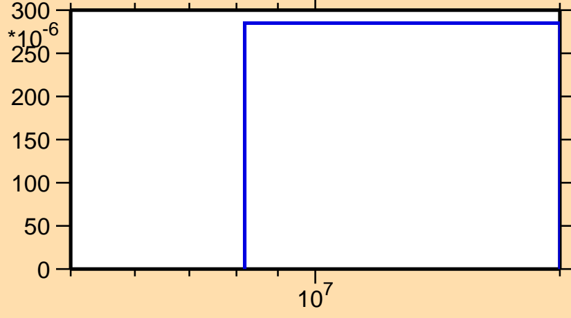
\sigma vs. E for ^{108}\text{Sb}(n,2np)
