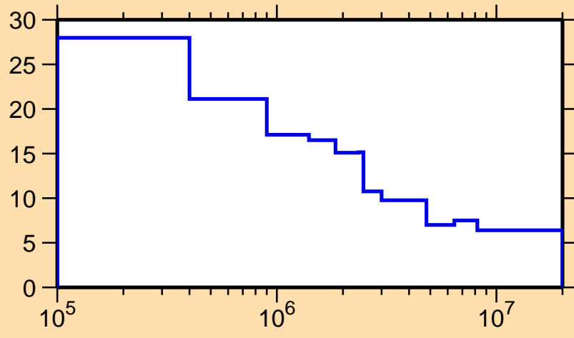
\Delta\sigma/\sigma vs. E for ^{108}\text{Sb}(n,\text{nonel.})
