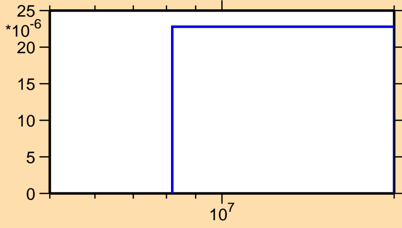
\sigma vs. E for ^{108}\text{Sb}(n,nd)
