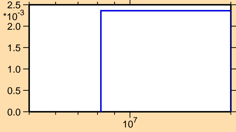
\sigma vs. E for ^{108}\text{Sb}(n,2n)
