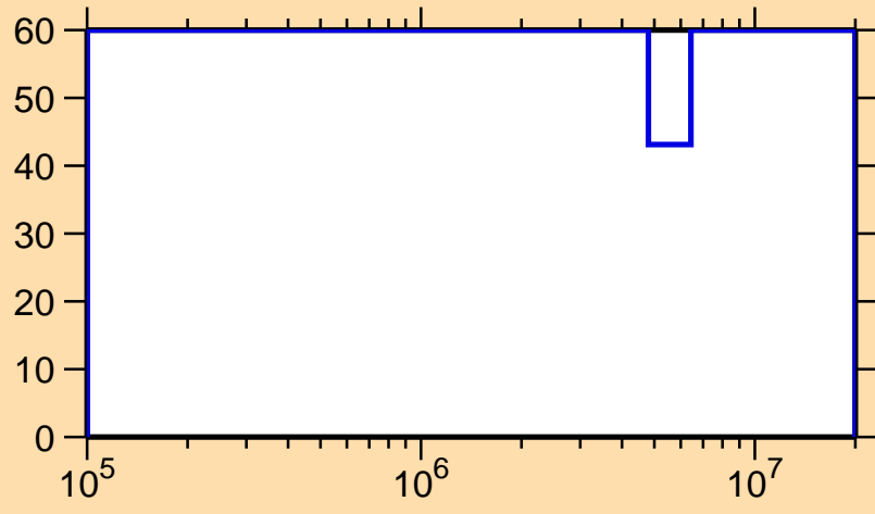
\Delta\sigma/\sigma vs. E for ^{108}\text{Sb}(n,n\text{cont.})
