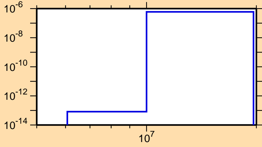
\sigma vs. E for ^{109}\text{Sb}(\text{mt117})
