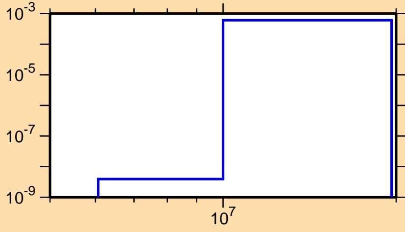
\sigma vs. E for ^{109}\text{Sb}(n,t)
