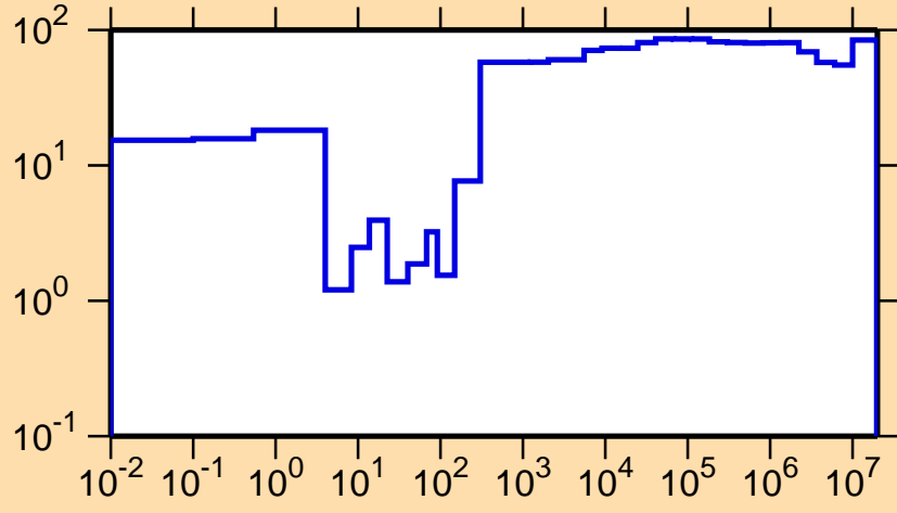
\Delta\sigma/\sigma vs. E for ^{109}\text{Sb}(n,\gamma)
