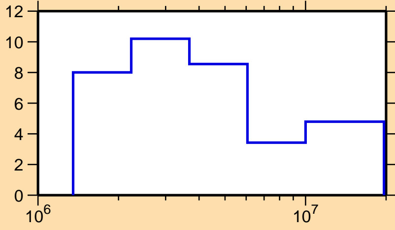
\Delta\sigma/\sigma vs. E for ^{109}\text{Sb}(n,el.)
