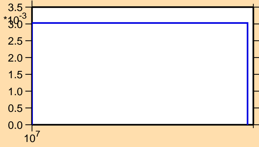
\sigma vs. E for ^{109}\text{Sb}(n,2n)
