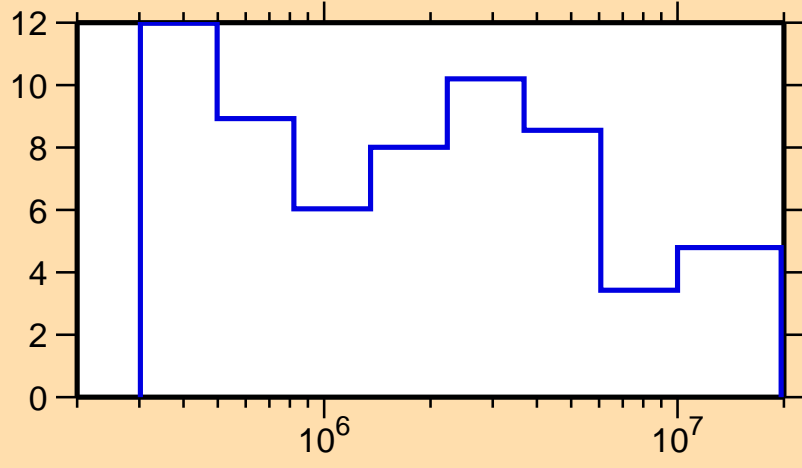
\Delta\sigma/\sigma vs. E for ^{109}\text{Sb}(n,\text{el.})
