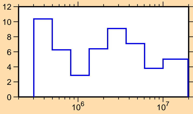
\Delta\sigma/\sigma vs. E for ^{109}\text{Sb}(n,\text{tot.})
