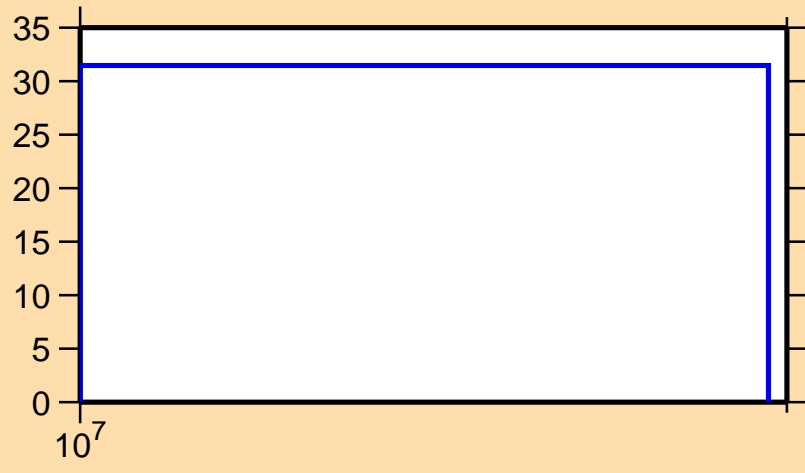
\Delta\sigma/\sigma vs. E for ^{109}\text{Sb}(n,\text{inel.})
