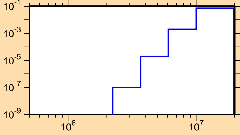
\sigma vs. E for ^{109}\text{Sb}(n,p\alpha)
