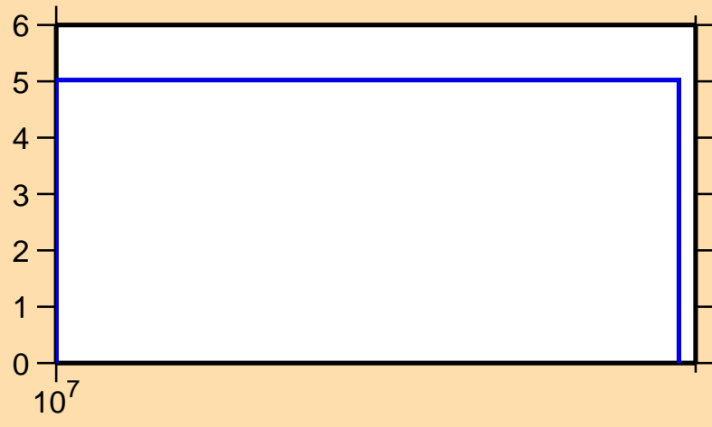
\Delta\sigma/\sigma vs. E for ^{109}\text{Sb}(n,\text{tot.})
