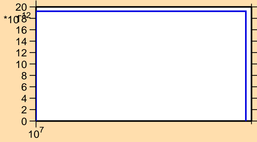
\sigma vs. E for ^{109}\text{Sb} (mt 34)
