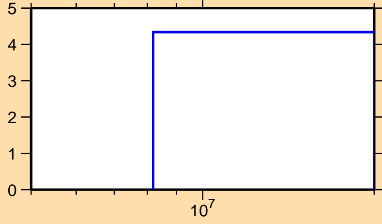
\Delta\sigma/\sigma vs. E for ^{109}\text{Sb}(n,\text{el.})
