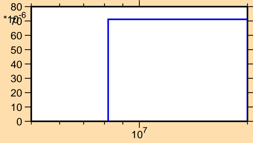
\sigma vs. E for ^{109}\text{Sb}(n,\text{pd})
