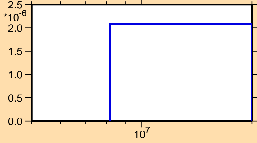
\sigma vs. E for ^{109}\text{Sb}(n,\text{nd})
