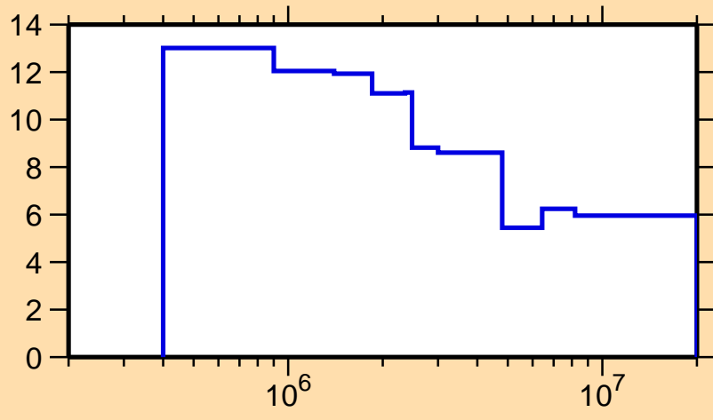
\Delta\sigma/\sigma vs. E for ^{109}\text{Sb}(n,\text{nonel.})
