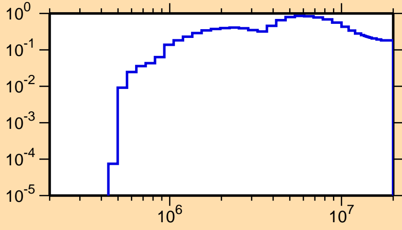
\sigma vs. E for ^{111}\text{Sb}(n,\text{inel.})
