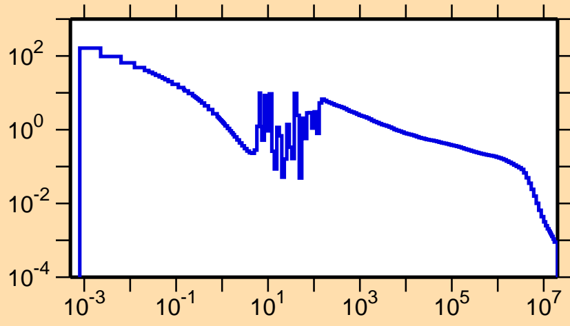
\sigma vs. E for ^{111}\text{Sb}(n,\gamma)
