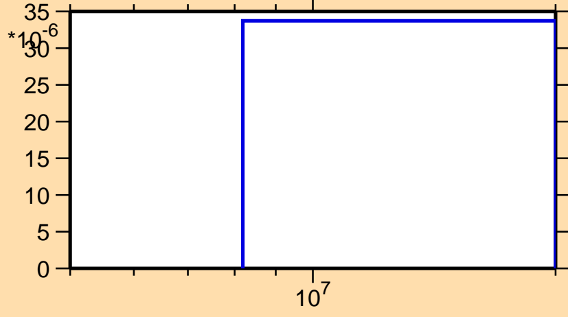
\sigma vs. E for ^{111}\text{Sb}(n,2np)
