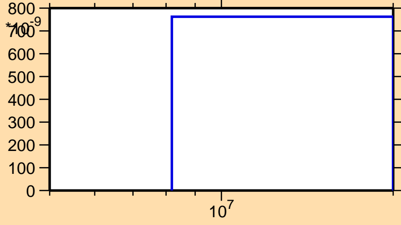
\sigma vs. E for ^{111}\text{Sb}(\text{mt } 45)
