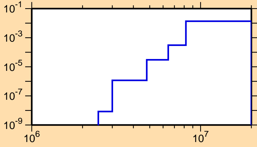
\sigma vs. E for ^{111}\text{Sb}(n,d)
