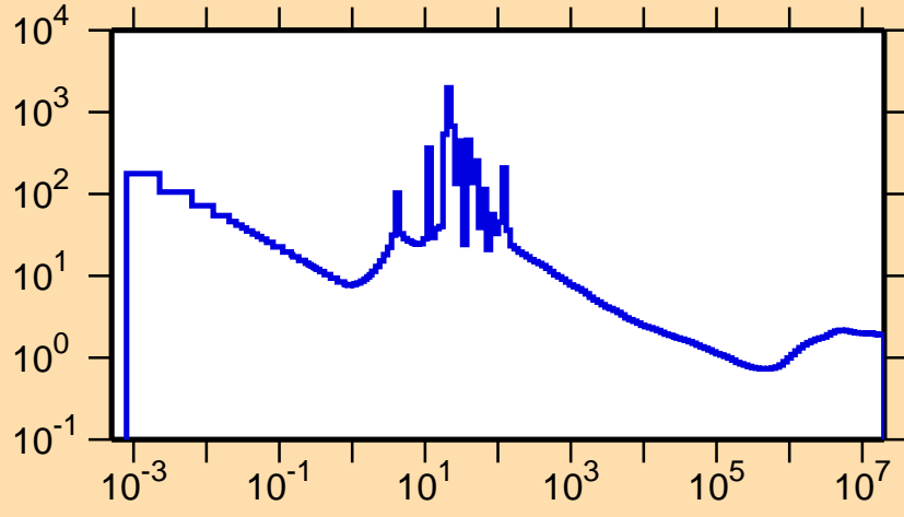
\sigma vs. E for ^{113}\text{Sb}(n,\text{nonel.})
