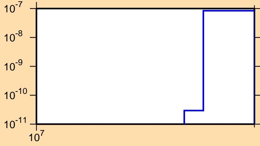
\sigma vs. E for ^{113}\text{Sb}(n,nt)
