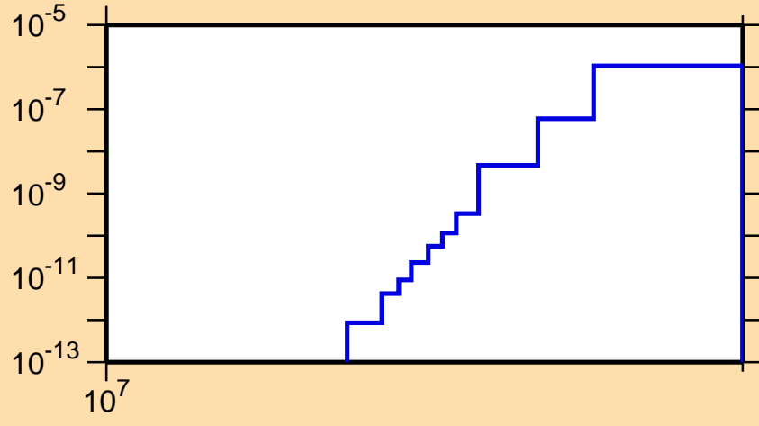
\sigma vs. E for ^{113}\text{Sb}(\text{mt } 45)
