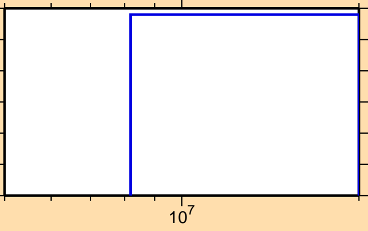
\sigma vs. E for ^{113}\text{Sb}(\text{mt } 45)
