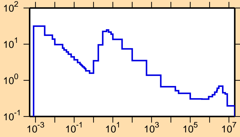
\sigma vs. E for ^{113}\text{Sb}(n,p)
