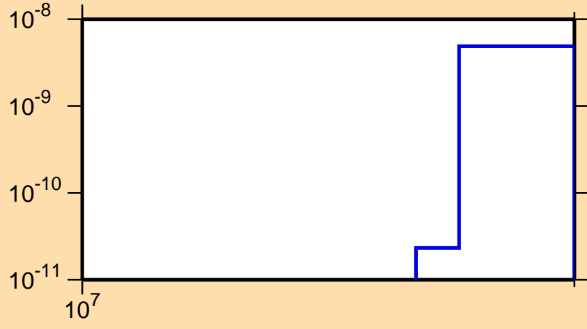
\sigma vs. E for ^{114}\text{Sb}(n,\text{pt})
