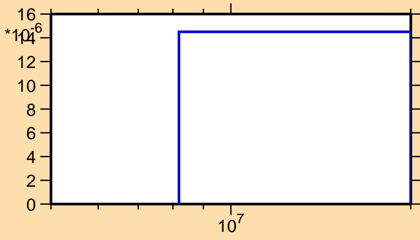
\sigma vs. E for ^{114}\text{Sb}(n,\text{nd})
