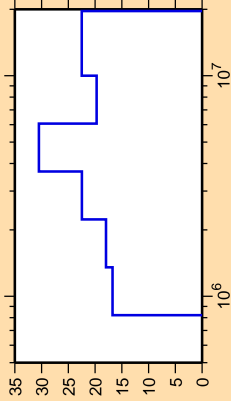
\Delta\sigma/\sigma vs. E for ^{115}\text{Sb}(n,n_3)
