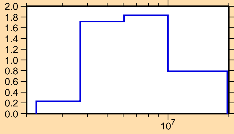
\sigma vs. E for ^{115}\text{Sb}(n,n\text{cont.})
