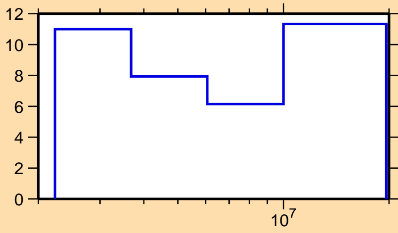
\Delta\sigma/\sigma vs. E for ^{115}\text{Sb}(n,n\text{cont.})
