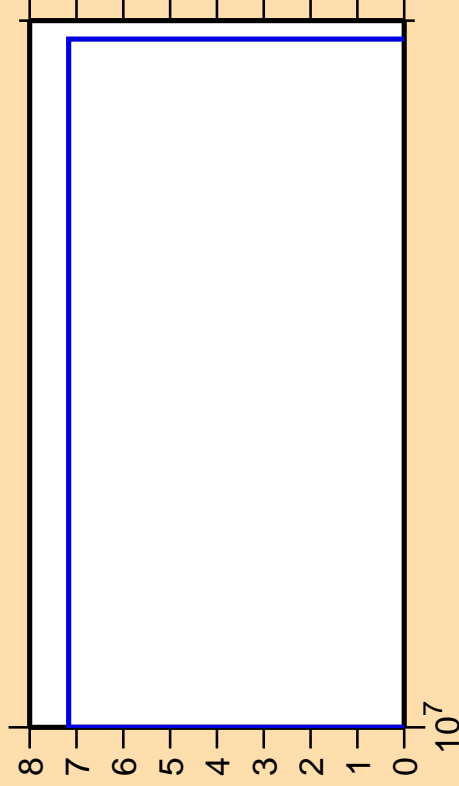
\Delta\sigma/\sigma vs. E for ^{115}\text{Sb}(\text{mt117})
