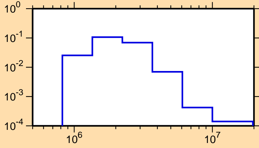
\sigma vs. E for ^{115}\text{Sb}(n,n_3)
