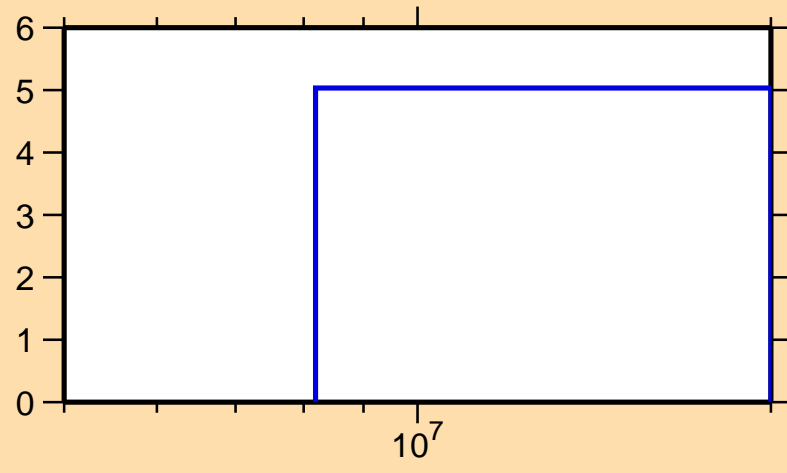
\Delta\sigma/\sigma vs. E for ^{115}\text{Sb}(n,\text{el.})
