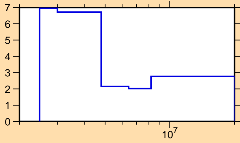
\Delta\sigma/\sigma vs. E for ^{115}\text{Sb}(n,\text{tot.})
