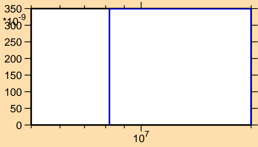
\sigma vs. E for ^{115}\text{Sb}(n,nd)
