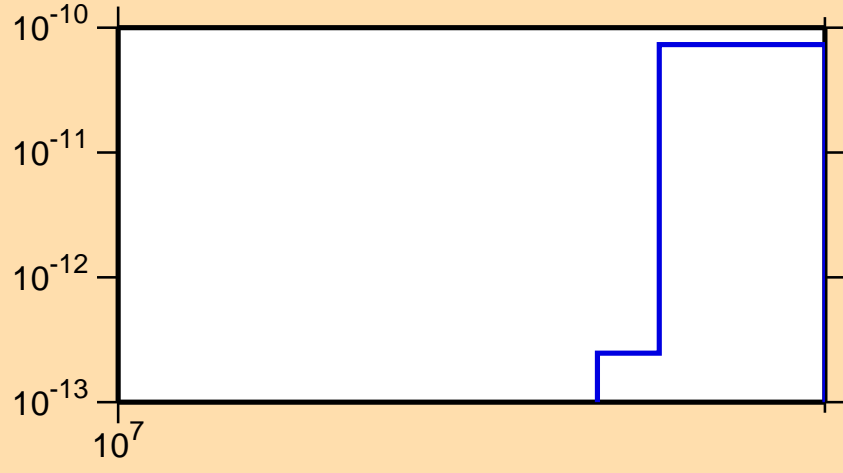
\sigma vs. E for ^{116}\text{Sb}(n,\text{pd})
