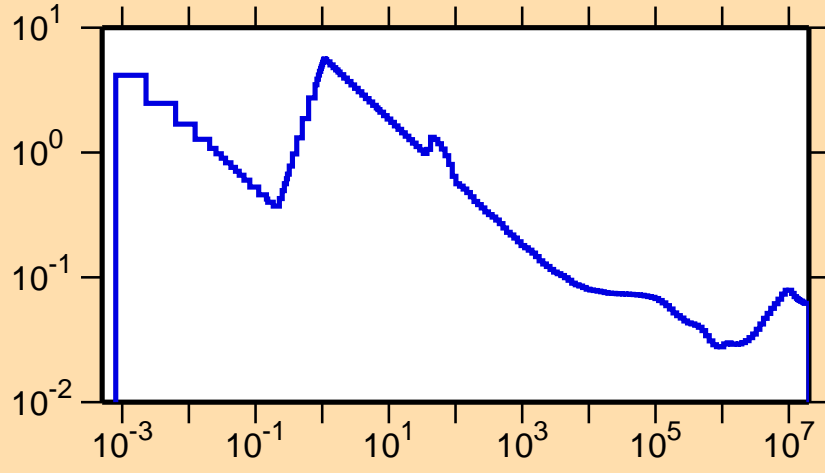
\sigma vs. E for ^{116}\text{Sb}(n,p)
