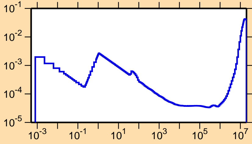
\sigma vs. E for ^{116}\text{Sb}(n,\alpha)
