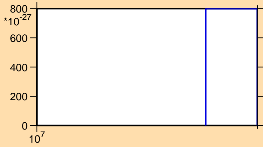
\sigma vs. E for ^{116}\text{Sb}(\text{mt 11})
