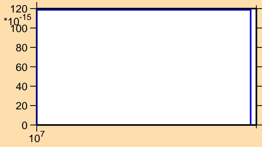
\sigma vs. E for ^{116}\text{Sb}(\text{mt117})
