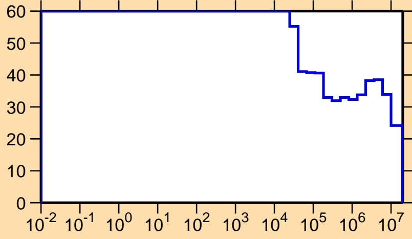
\Delta\sigma/\sigma vs. E for ^{116}\text{Sb}(n,p)
