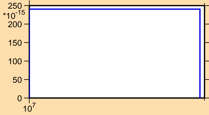
\sigma vs. E for ^{116}\text{Sb} (mt 45)
