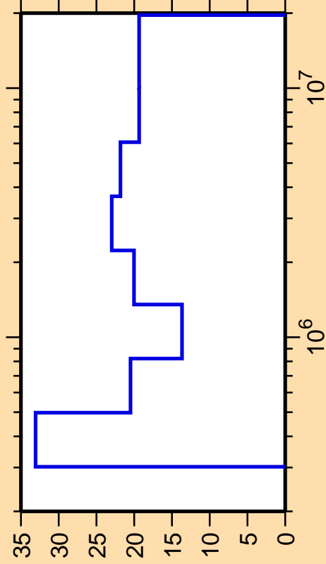
\Delta\sigma/\sigma vs. E for ^{116}\text{Sb}(n,n_3)
