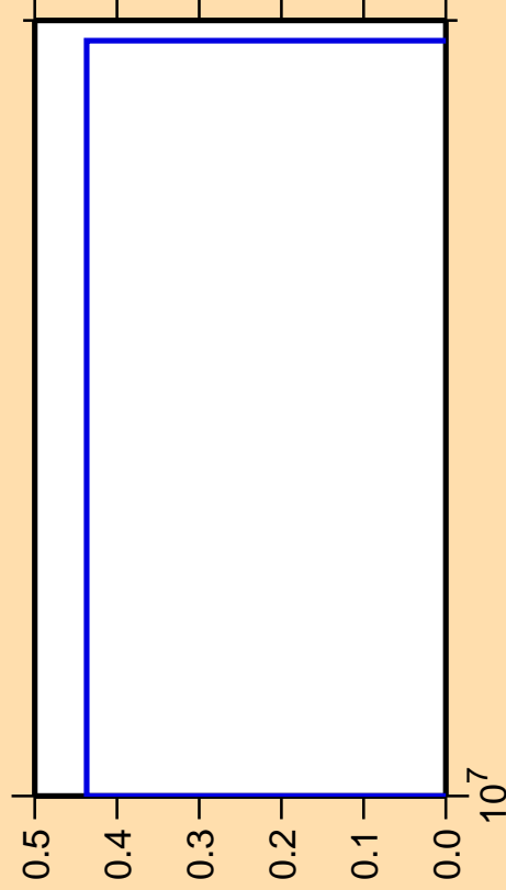
\Delta\sigma/\sigma vs. E for ^{116}\text{Sb} (mt 45)
