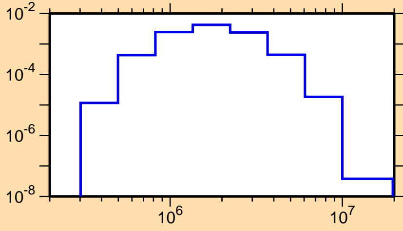
\sigma vs. E for ^{116}\text{Sb}(n,n_3)
