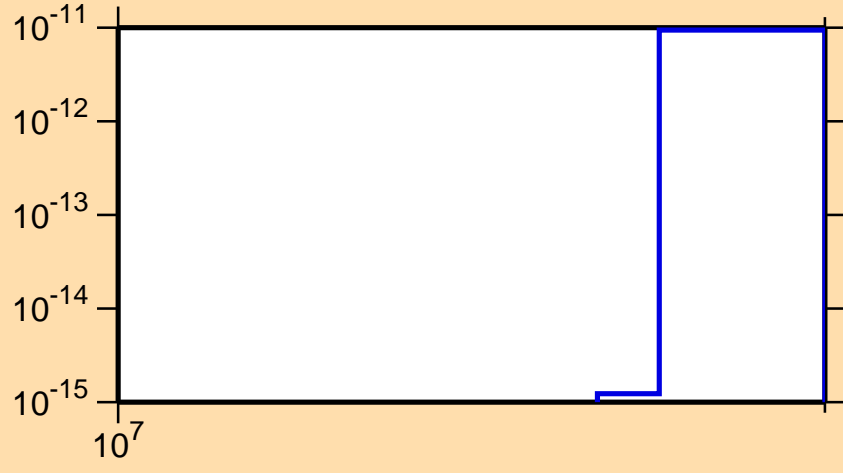
\sigma vs. E for ^{116}\text{Sb}(\text{mt } 34)
