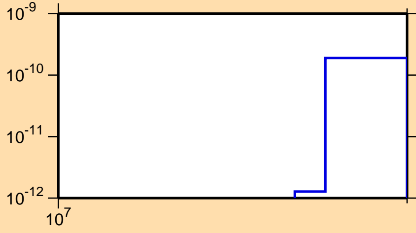
\sigma vs. E for ^{116}\text{Sb}(n,pd)
