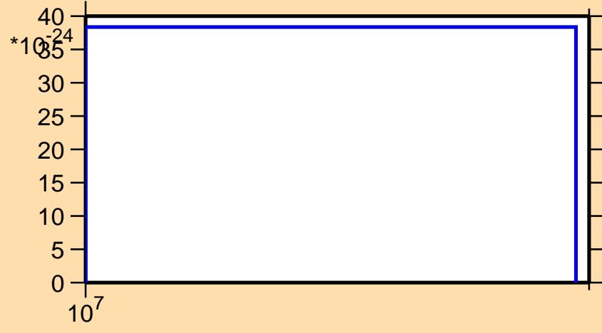
\sigma vs. E for ^{116}\text{Sb} (mt 11)
