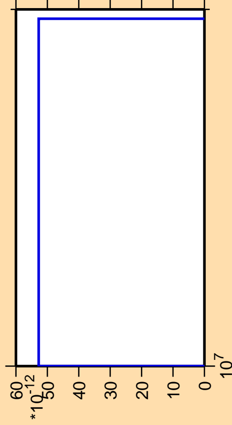
\Delta\sigma/\sigma vs. E for ^{116}\text{Sb} (mt 11)
