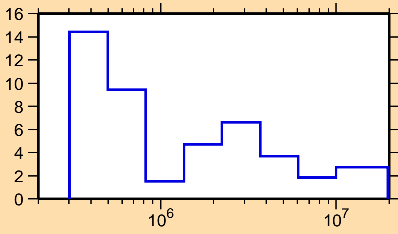
\Delta\sigma/\sigma vs. E for ^{116}\text{Sb}(n,\text{tot.})
