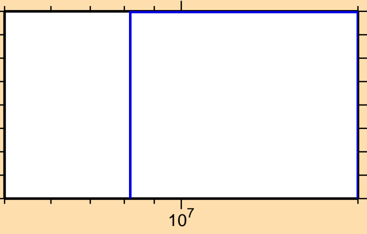
\sigma vs. E for ^{116}\text{Sb}(\text{mt } 45)
