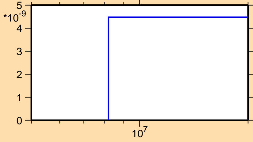
\sigma vs. E for ^{118}\text{Sb}(n,p\alpha)
