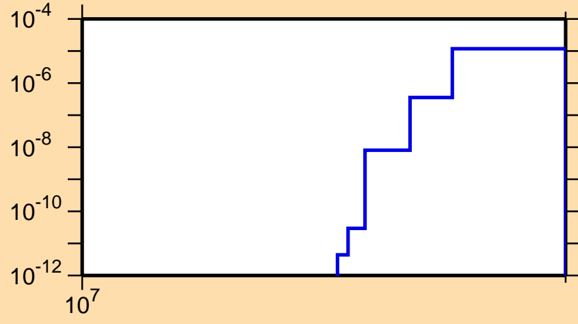
\sigma vs. E for ^{119}\text{Sb}(n,nd)
