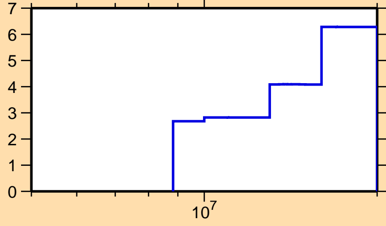
\Delta\sigma/\sigma vs. E for ^{119}\text{Sb}(n,\text{el.})
