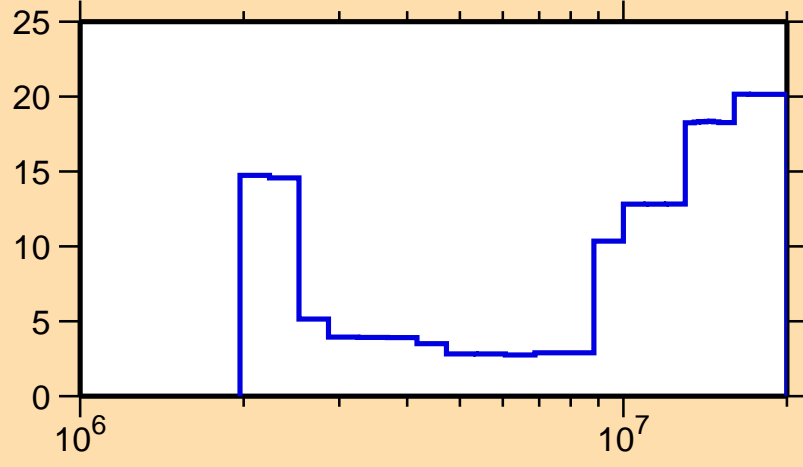
\Delta\sigma/\sigma vs. E for ^{119}\text{Sb}(n,n\text{cont.})
