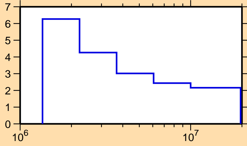
\Delta\sigma/\sigma vs. E for ^{119}\text{Sb}(n,nonel.)
