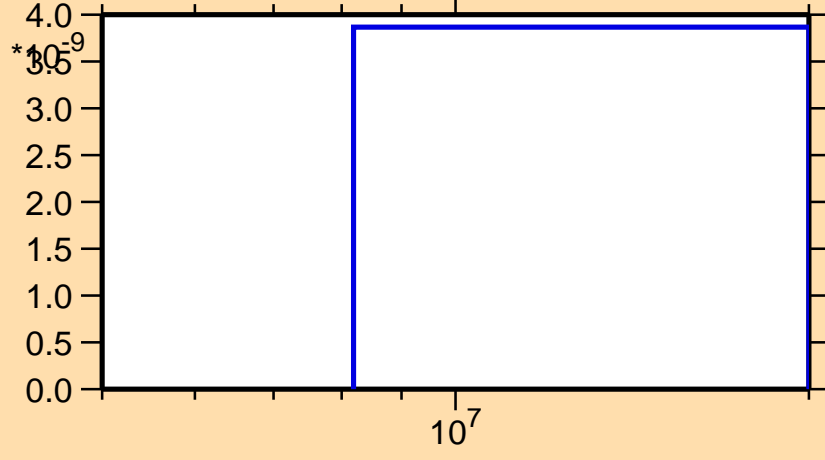
\sigma vs. E for ^{119}\text{Sb}(n,nt)
