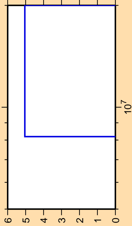
\Delta\sigma/\sigma vs. E for ^{119}\text{Sb}(n,2n)
