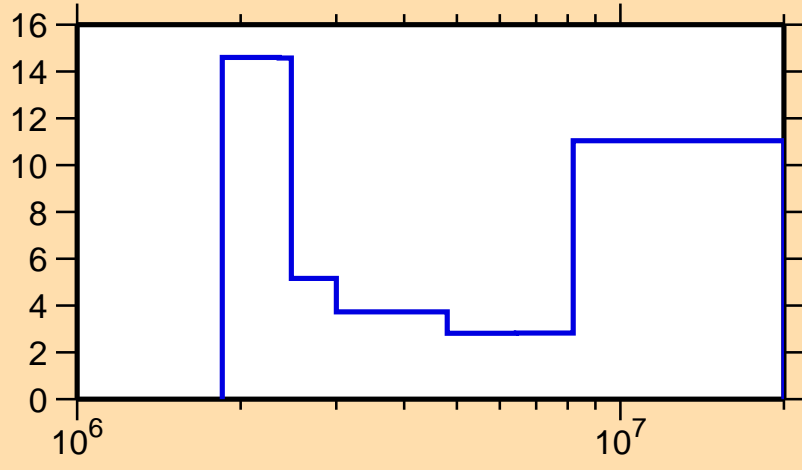
\Delta\sigma/\sigma vs. E for ^{119}\text{Sb}(n,n\text{cont.})
