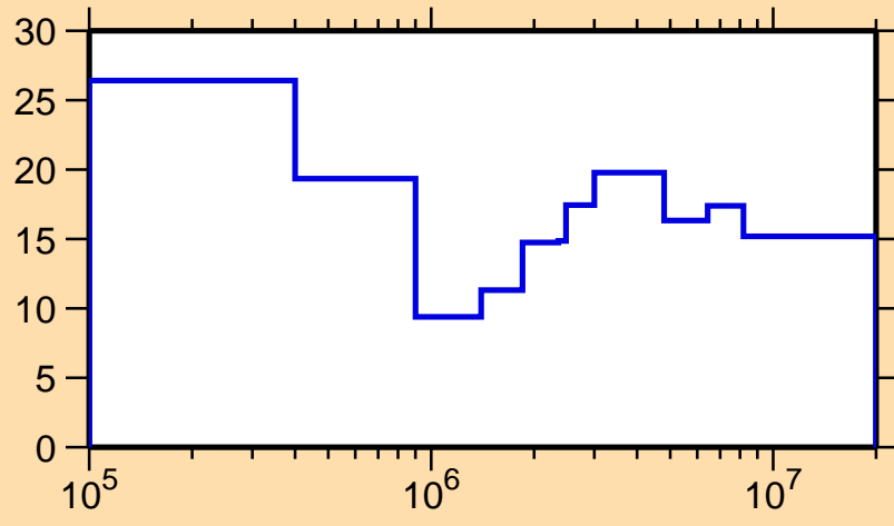
\Delta\sigma/\sigma vs. E for ^{119}\text{Sb}(n,n_1)
