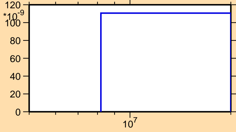
\sigma vs. E for ^{119}\text{Sb}(n,\text{nd})
