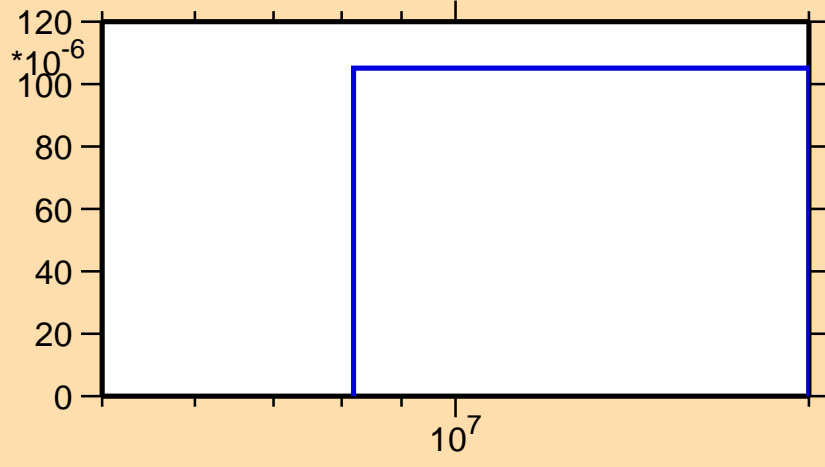
\sigma vs. E for ^{119}\text{Sb}(n,t)
