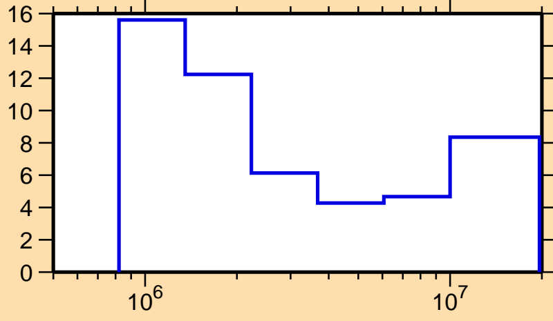
\Delta\sigma/\sigma vs. E for ^{120}\text{Sb}(n,n\text{cont.})
