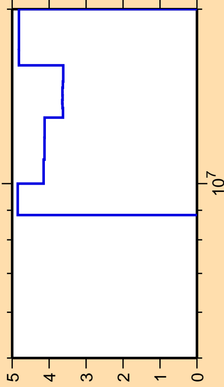
\Delta\sigma/\sigma vs. E for ^{123}\text{Sb}(n,2n)
