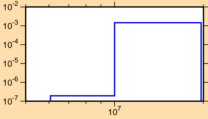
\sigma vs. E for ^{123}\text{Sb}(n,d)
