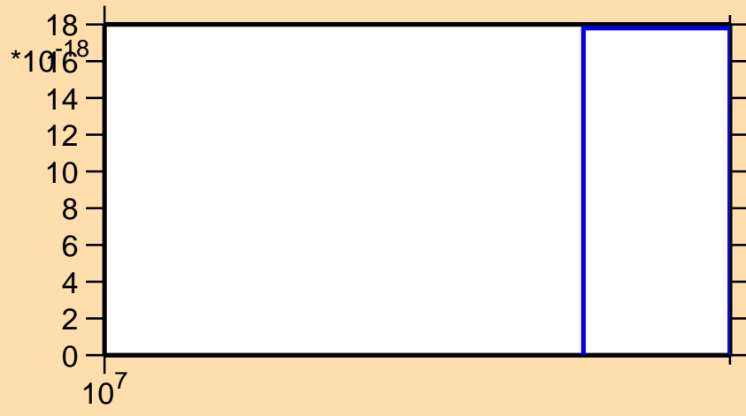
\sigma vs. E for ^{124}\text{Sb} (mt 11)
