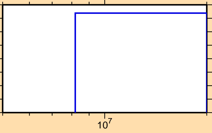
\sigma vs. E for ^{124}\text{Sb}(n,2np)
