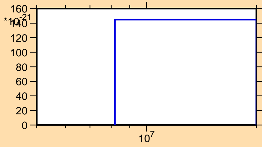
\sigma vs. E for ^{124}\text{Sb}(\text{mt } 11)
