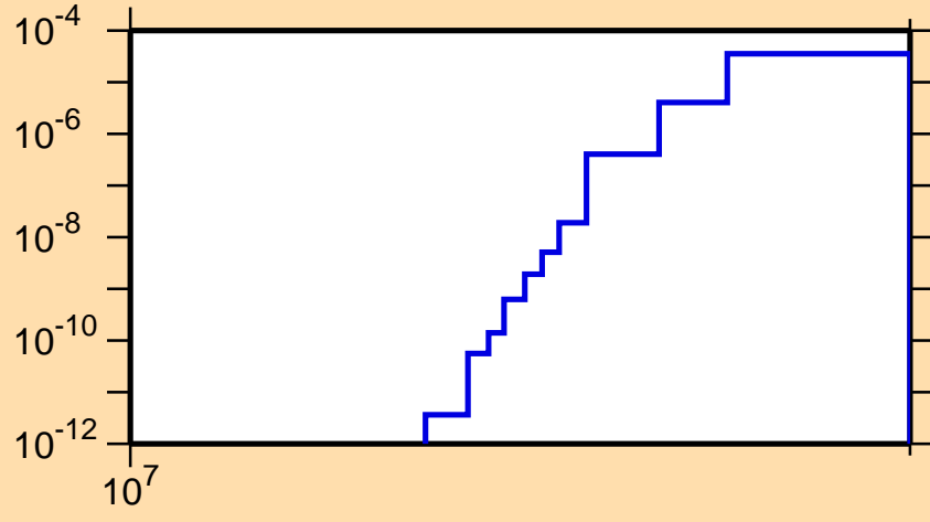
\sigma vs. E for ^{124}\text{Sb}(n,\text{nd})
