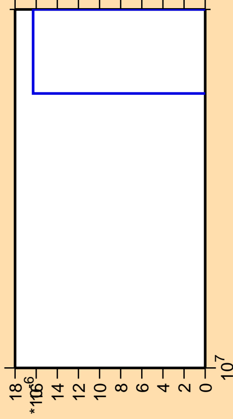
\Delta\sigma/\sigma vs. E for ^{124}\text{Sb} (mt 11)
