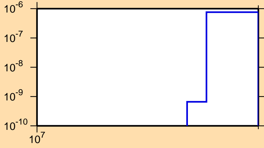
\sigma vs. E for ^{124}\text{Sb}(n,nt)
