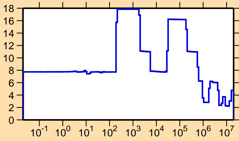
\Delta\sigma/\sigma vs. E for ^{124}\text{Sb}(n,\text{el.})
