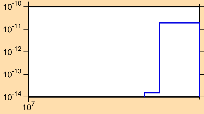
\sigma vs. E for ^{124}\text{Sb}(n,\text{He}3)
