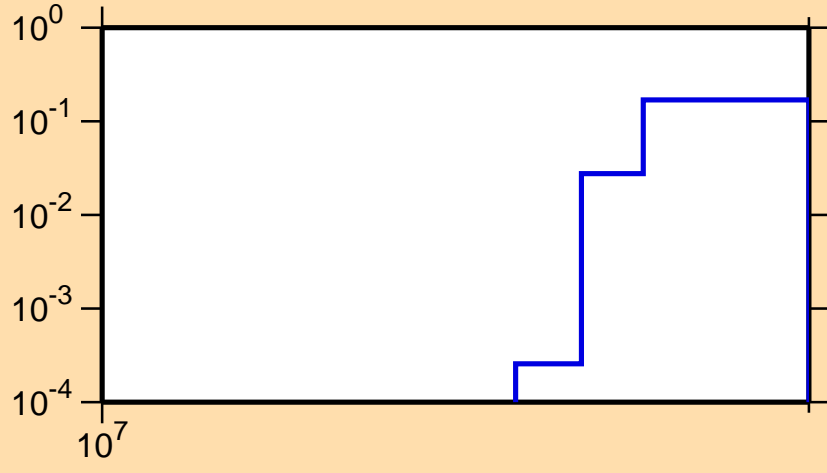
\sigma vs. E for ^{124}\text{Sb}(n,3n)
