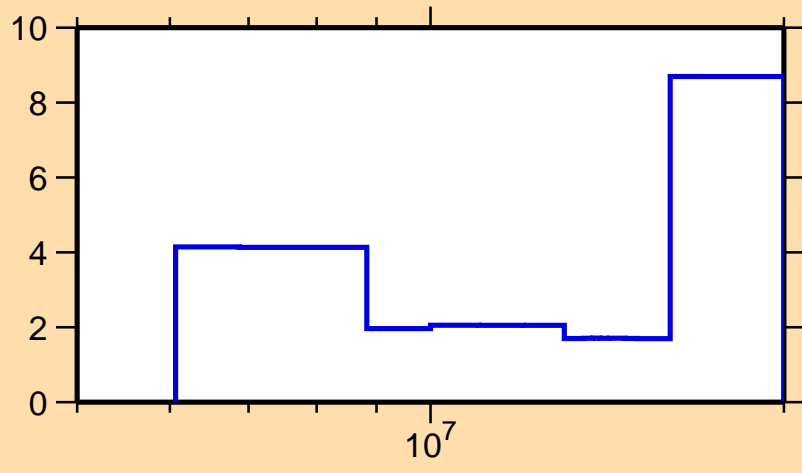
\Delta\sigma/\sigma vs. E for ^{124}\text{Sb}(n,2n)
