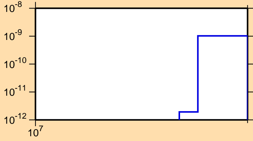
\sigma vs. E for ^{124}\text{Sb}(n,2n\alpha)
