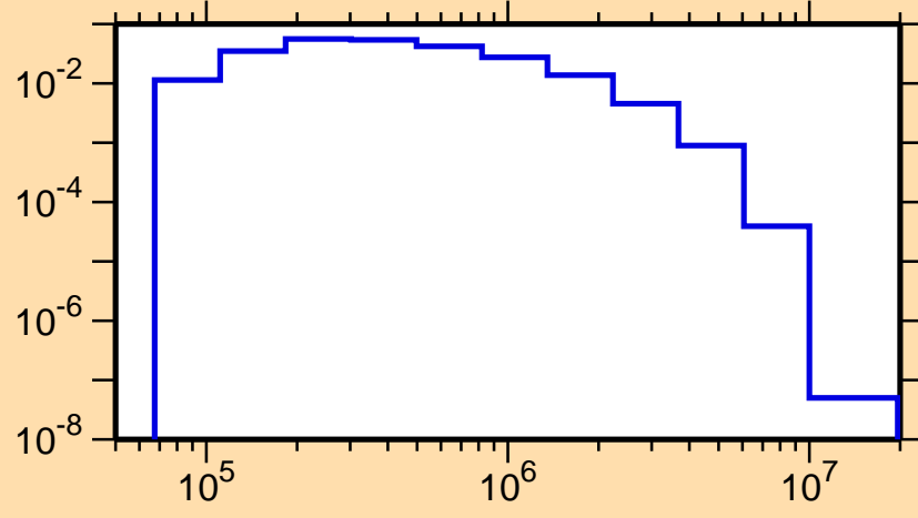
\sigma vs. E for ^{124}\text{Sb}(n,n_4)
