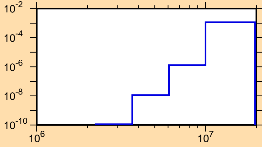
\sigma vs. E for ^{124}\text{Sb}(n,\alpha)
