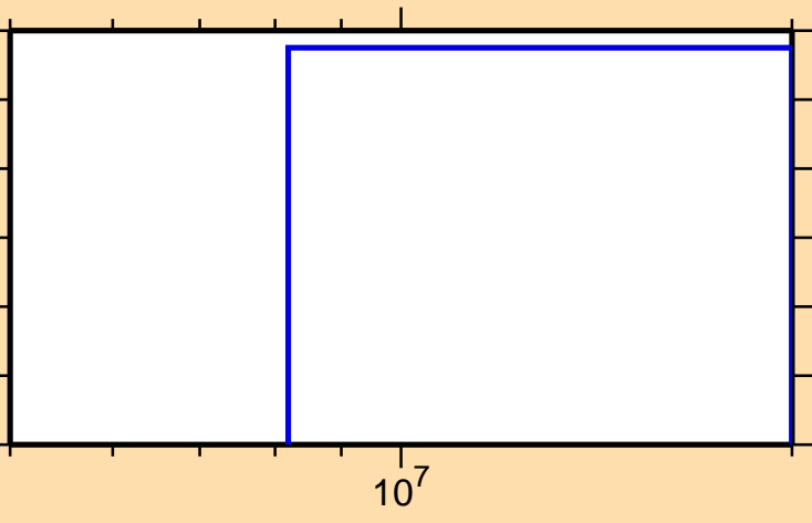
\sigma vs. E for ^{124}\text{Sb}(n,2np)
