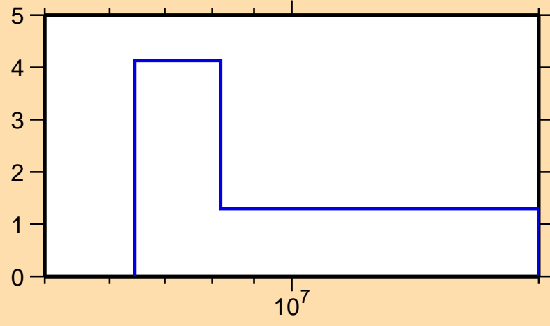
\Delta\sigma/\sigma vs. E for ^{124}\text{Sb}(n,2n)
