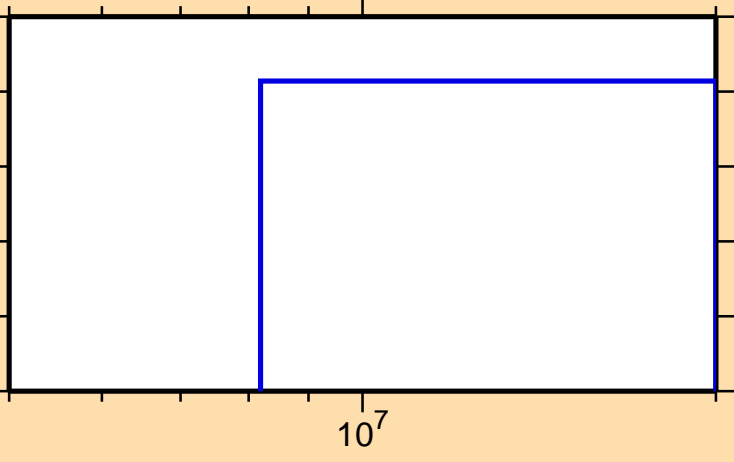
\sigma vs. E for ^{126}\text{Sb}(n,nt)
