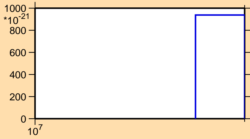
\sigma vs. E for ^{127}\text{Sb} (mt 11)
