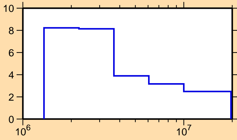
\Delta\sigma/\sigma vs. E for ^{127}\text{Sb}(n, tot.)
