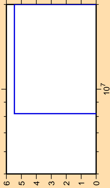
\Delta\sigma/\sigma vs. E for ^{127}\text{Sb}(n,2n)
