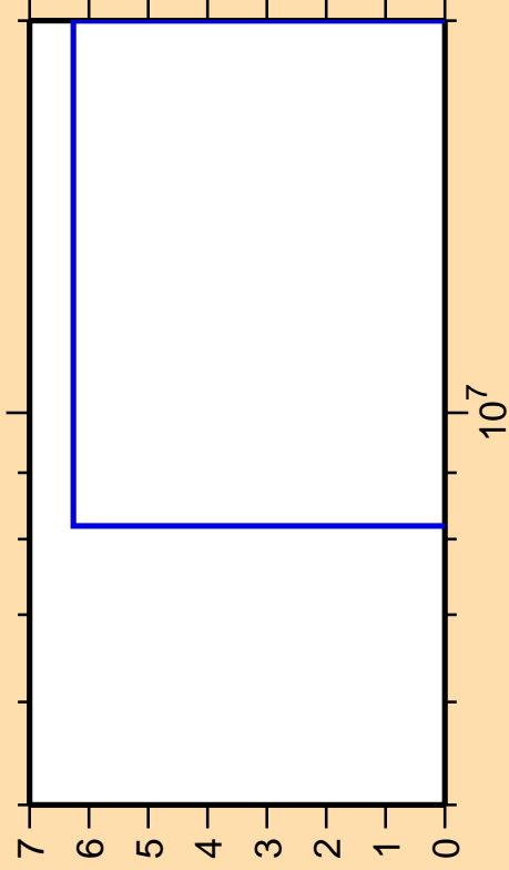
\Delta\sigma/\sigma vs. E for ^{127}\text{Sb}(n,2np)
