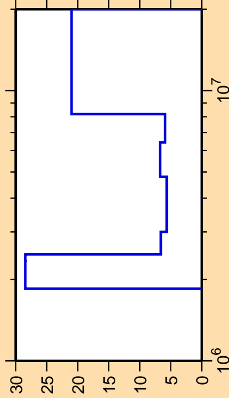
\Delta\sigma/\sigma vs. E for ^{127}\text{Sb}(n,n\text{cont.})
