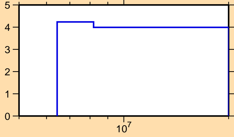
\Delta\sigma/\sigma vs. E for ^{127}\text{Sb}(n,\text{el.})
