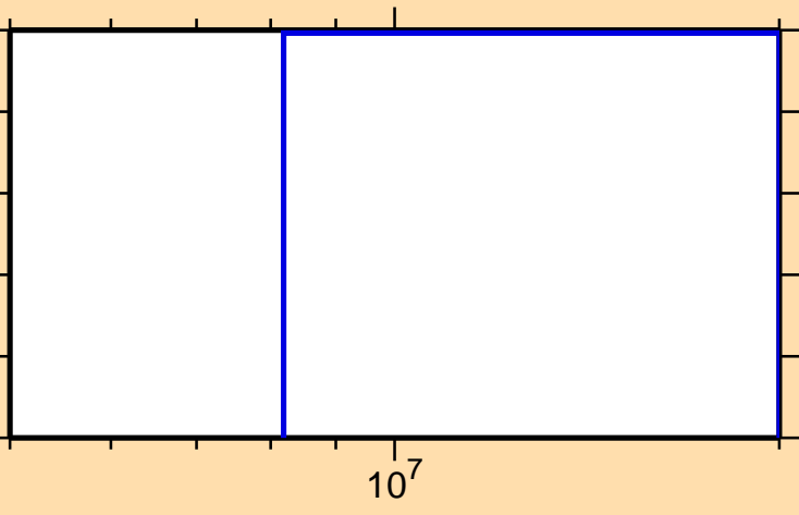
\sigma vs. E for ^{127}\text{Sb}(n,3n)
