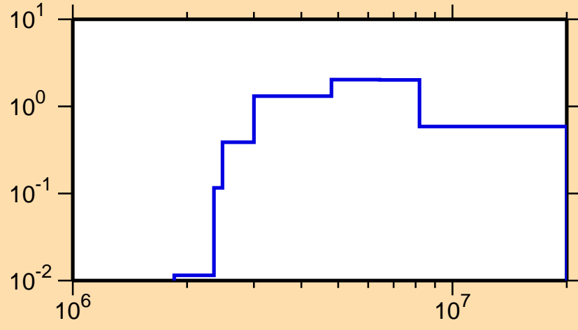
\sigma vs. E for ^{127}\text{Sb}(n,n\text{cont.})
