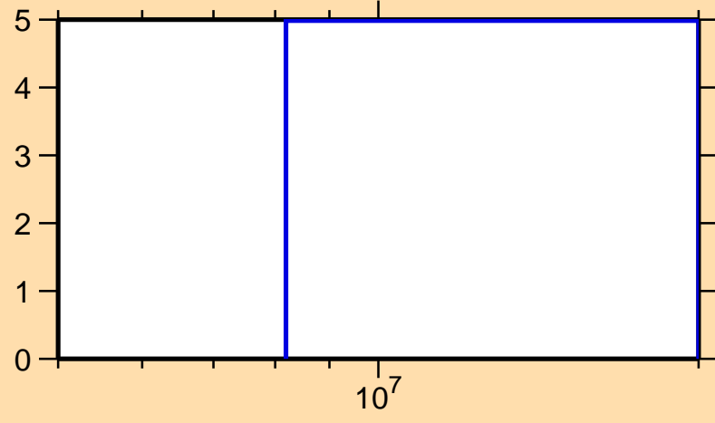
\Delta\sigma/\sigma vs. E for ^{127}\text{Sb}(n,\text{nonel.})
