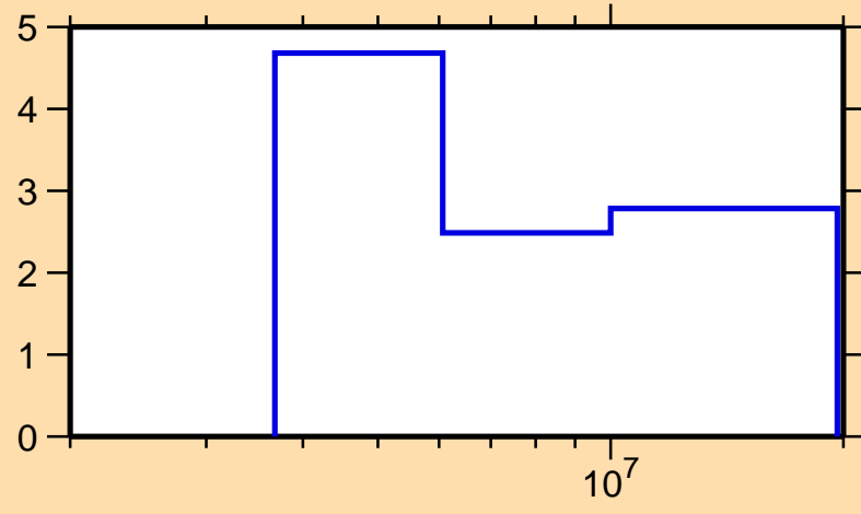
\Delta\sigma/\sigma vs. E for ^{128}\text{Sb}(n,\text{tot.})
