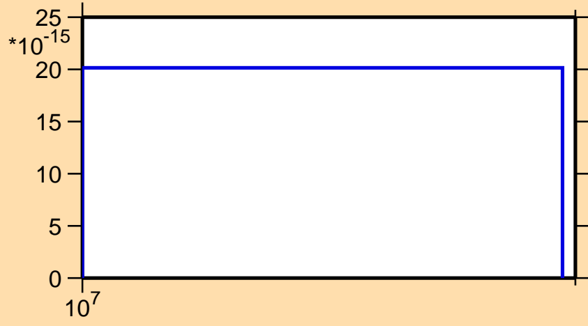
\sigma vs. E for ^{128}\text{Sb}(n,2n\alpha)
