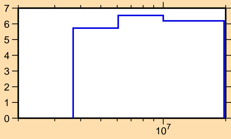
\Delta\sigma/\sigma vs. E for ^{128}\text{Sb}(n,\text{nonel.})
