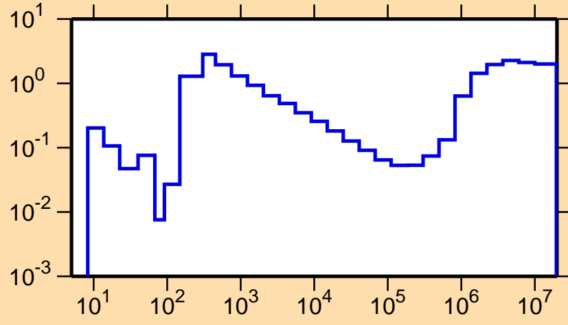
\sigma vs. E for ^{128}\text{Sb}(n,\text{nonel.})
