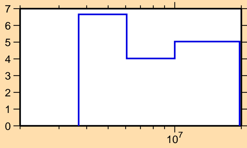
\Delta\sigma/\sigma vs. E for ^{128}\text{Sb}(n,\text{el.})
