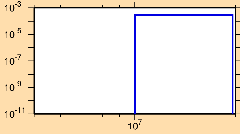
\sigma vs. E for ^{128}\text{Sb}(n,np)
