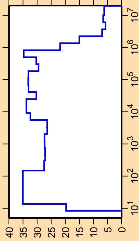
\Delta\sigma/\sigma vs. E for ^{128}\text{Sb}(n,\text{nonel.})
