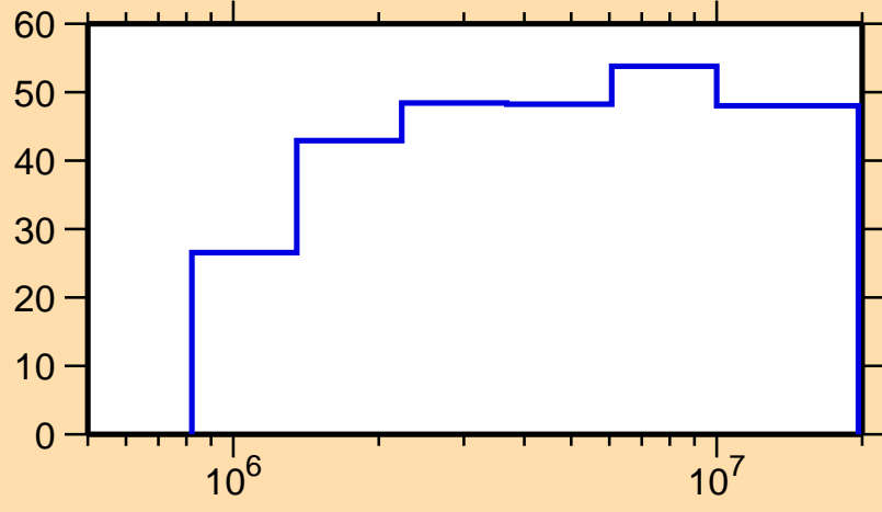
\Delta\sigma/\sigma vs. E for ^{128}\text{Sb}(n,n_1)
