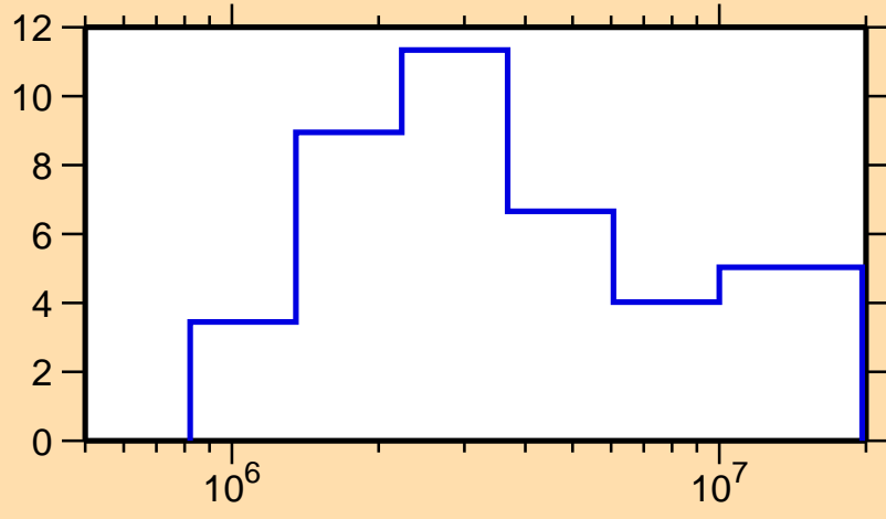
\Delta\sigma/\sigma vs. E for ^{128}\text{Sb}(n,el.)
