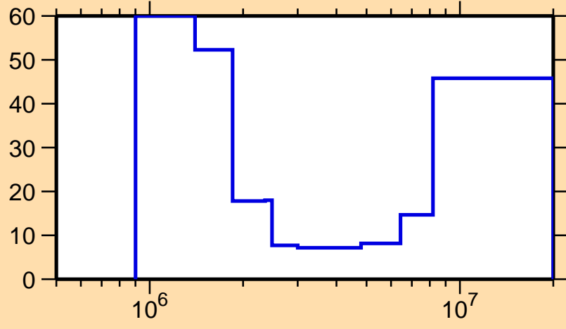
\Delta\sigma/\sigma vs. E for ^{128}\text{Sb}(n,n\text{cont.})
