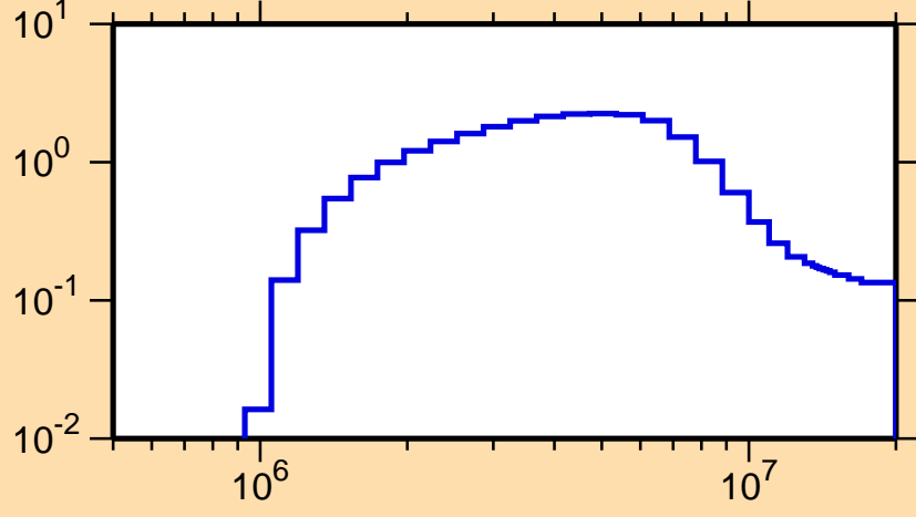
\sigma vs. E for ^{128}\text{Sb}(n,n\text{cont.})
