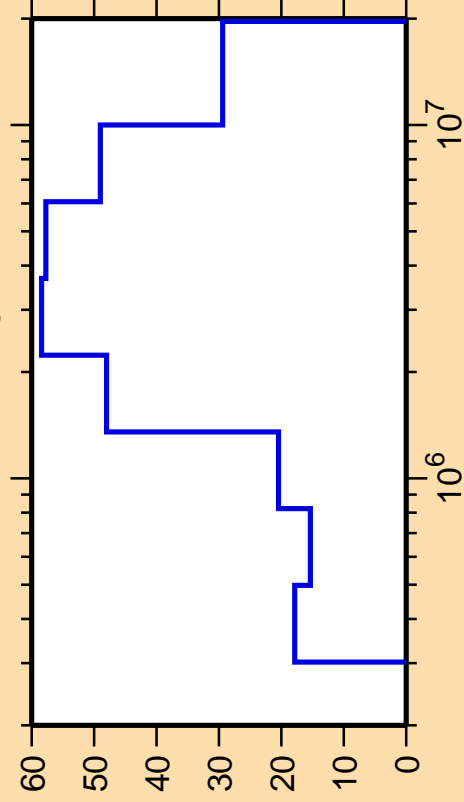
\Delta\sigma/\sigma vs. E for ^{128}\text{Sb}(n,n_3)
