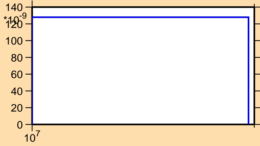
\sigma vs. E for ^{128}\text{Sb}(n,nd)
