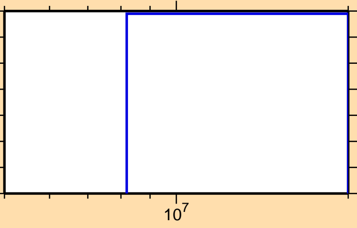
\sigma vs. E for ^{128}\text{Sb}(n,np)
