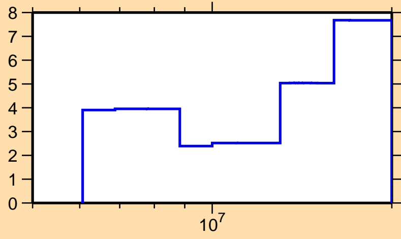
\Delta\sigma/\sigma vs. E for ^{129}\text{Sb}(n,\text{tot.})
