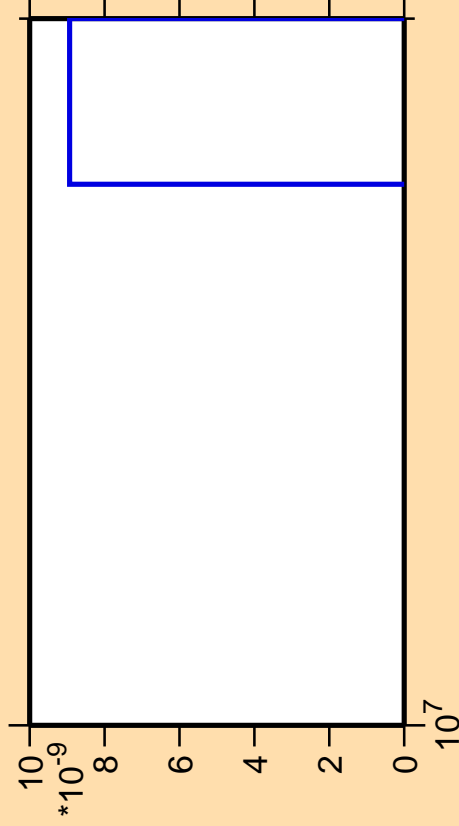
\Delta\sigma/\sigma vs. E for ^{129}\text{Sb} (mt 11)
