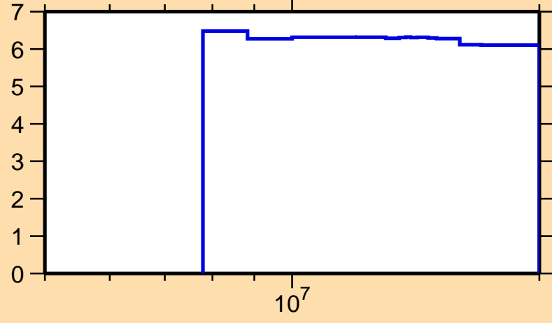
\Delta\sigma/\sigma vs. E for ^{129}\text{Sb}(n,\text{nonel.})
