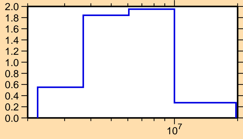
\sigma vs. E for ^{129}\text{Sb}(n,n\text{cont.})
