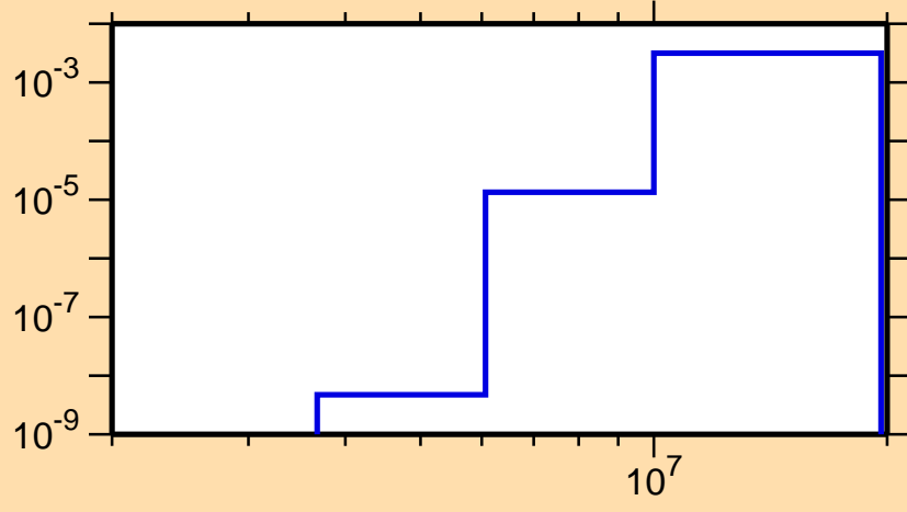
\sigma vs. E for ^{129}\text{Sb}(n,p)
