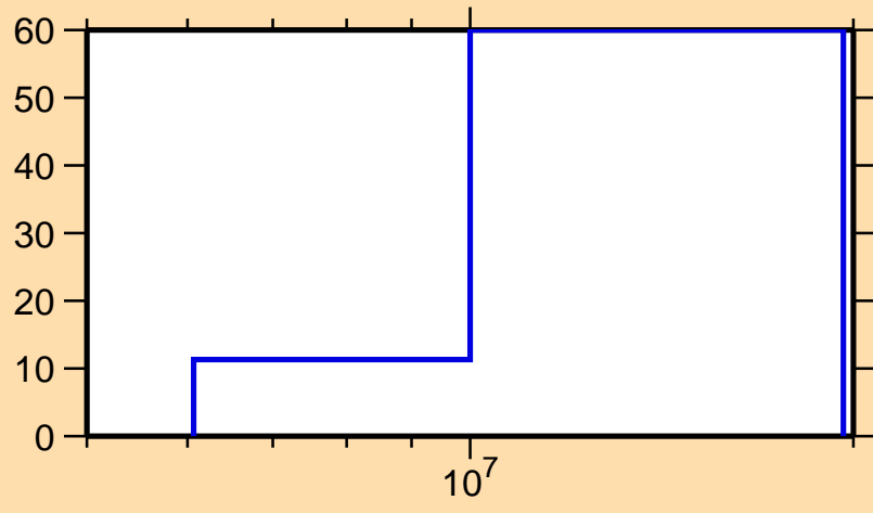
\Delta\sigma/\sigma vs. E for ^{129}\text{Sb}(n,n\text{cont.})
