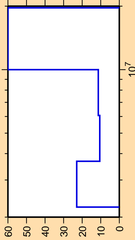
\Delta\sigma/\sigma vs. E for ^{129}\text{Sb}(n,n\text{cont.})
