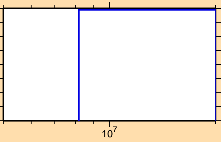
\sigma vs. E for ^{129}\text{Sb}(n,n\alpha)
